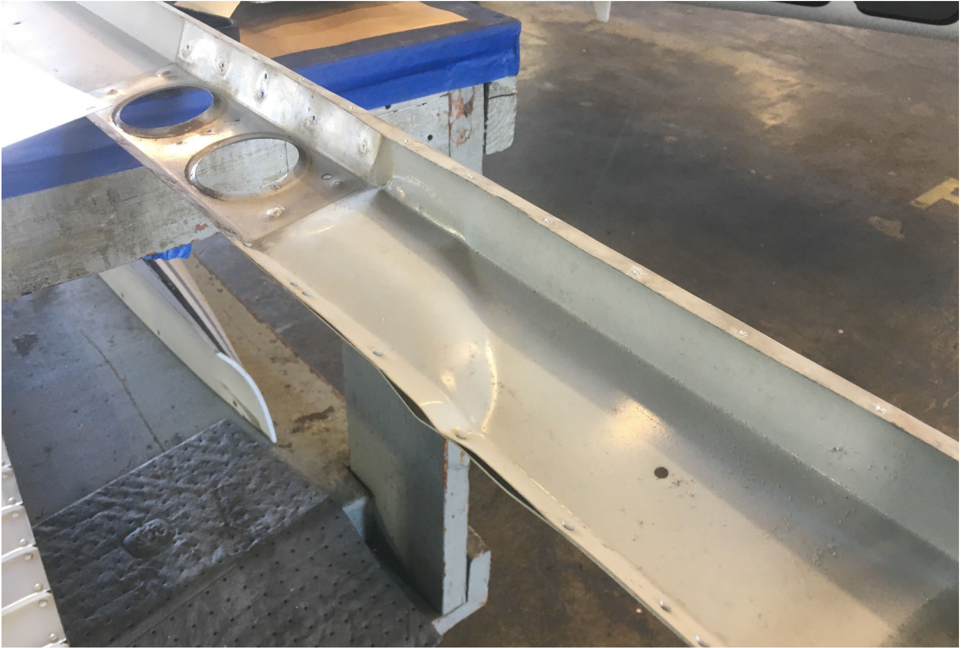
Photo 1 – Post-accident view of damage to left wing auxiliary spar (Courtesy of FAA)
