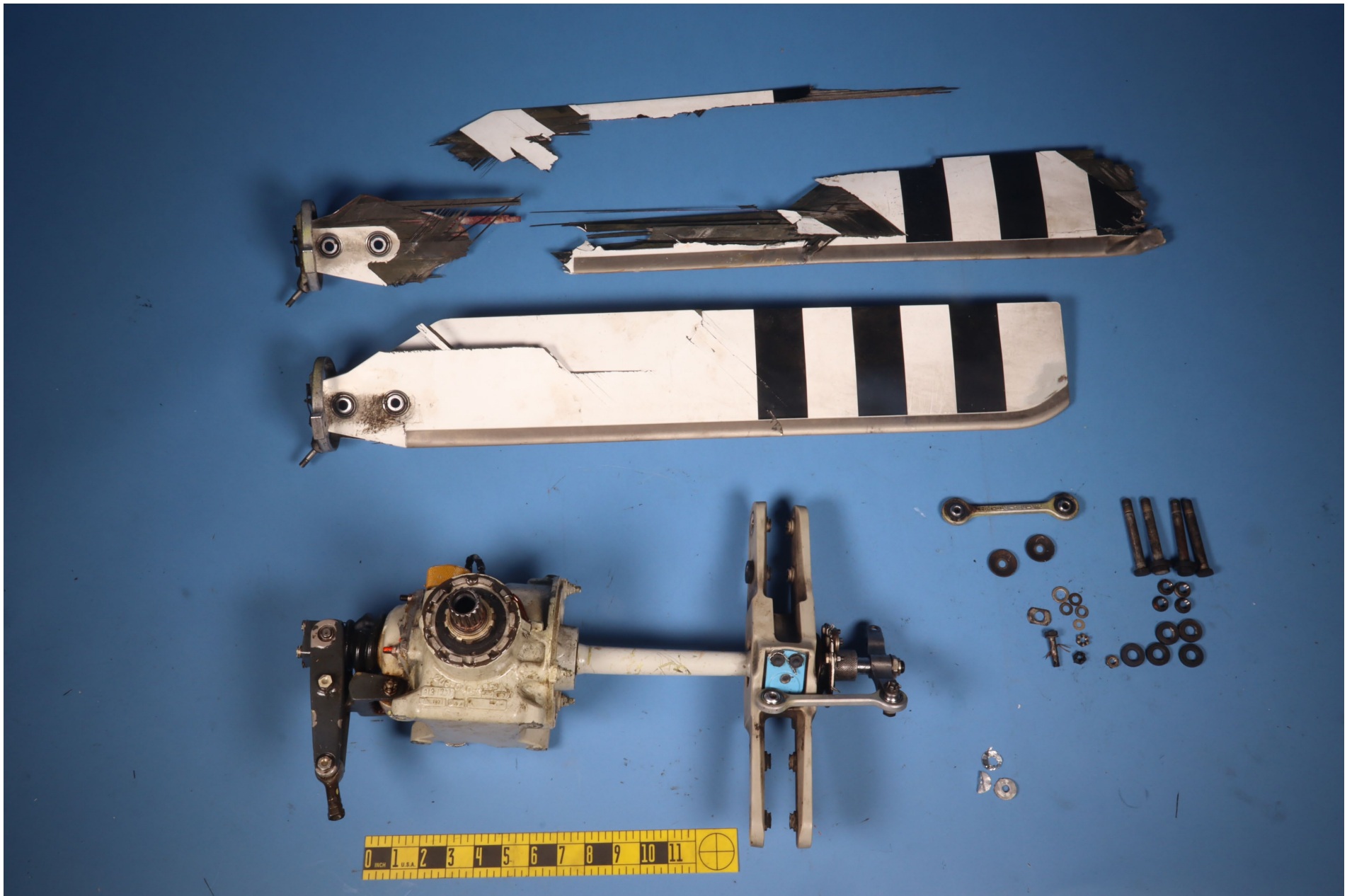
Photo 4 – Components received by the National Transportation Safety Board’s Materials laboratory.
