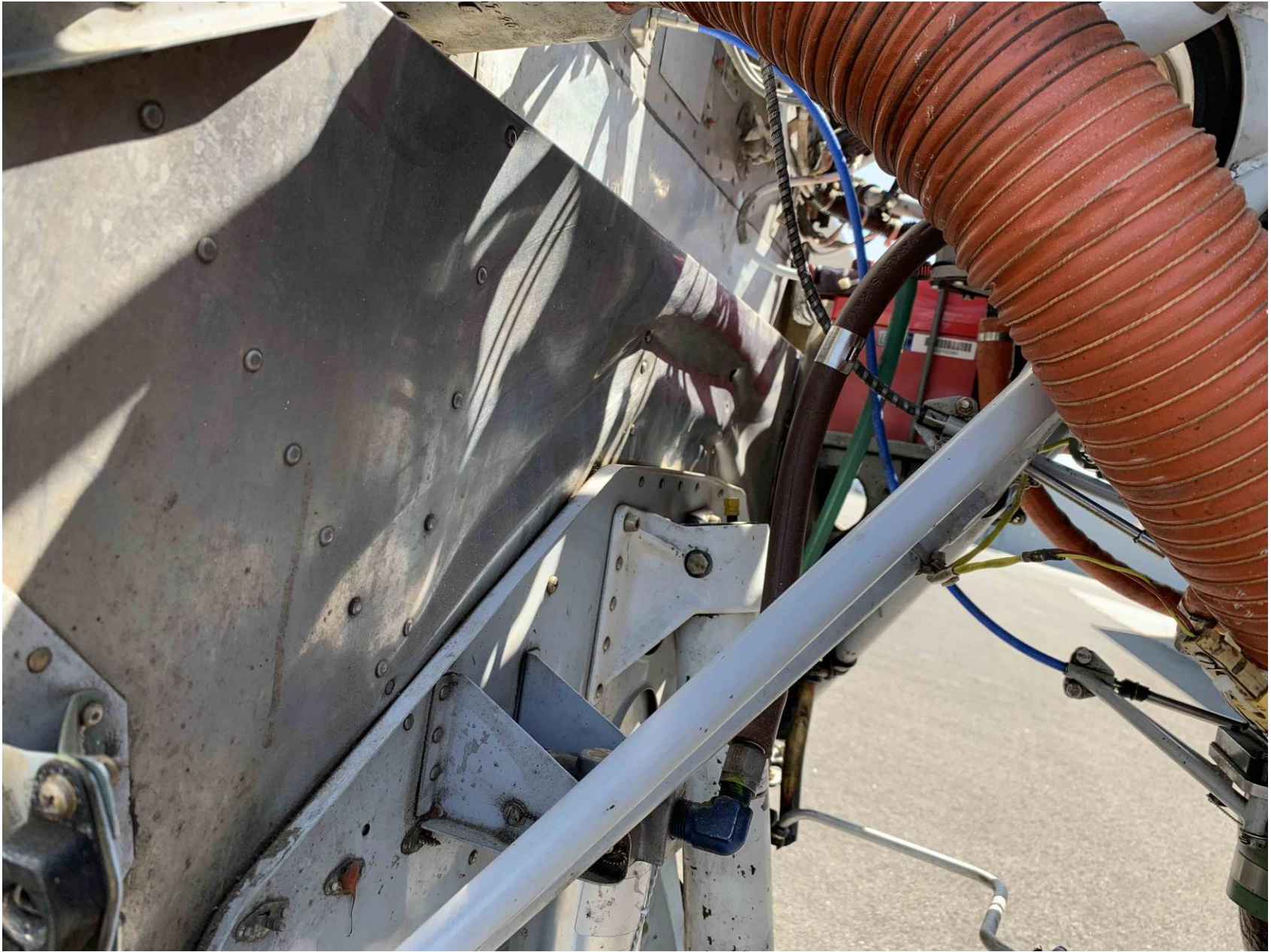
Photo 8 - Firewall and nose landing gear attachment. (Courtesy of the operator)
