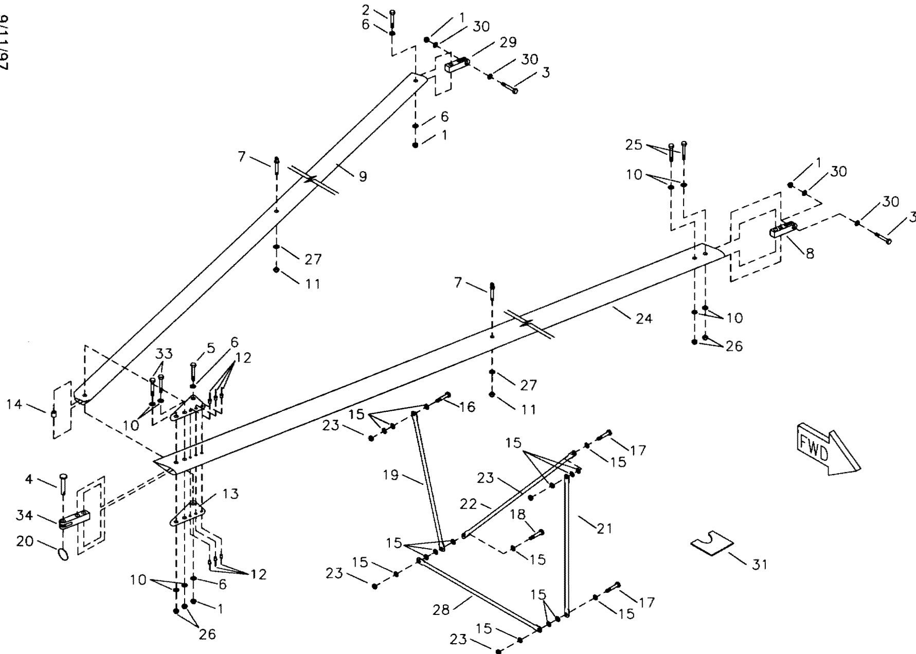
RANS S-4/5 COYOTE AIRFOIL LIFT STRUTS
