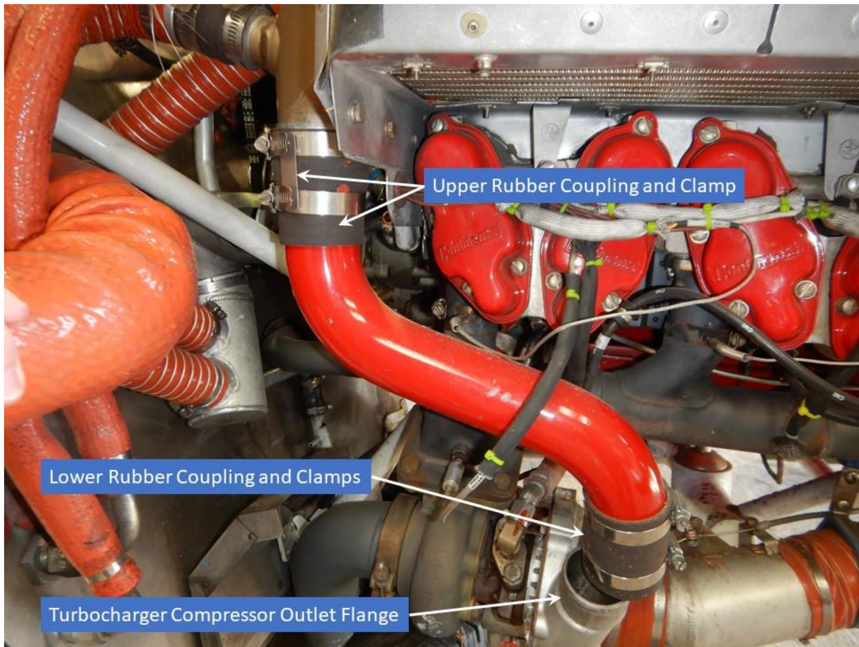
Photo 1 – Right side of engine and induction tube.
