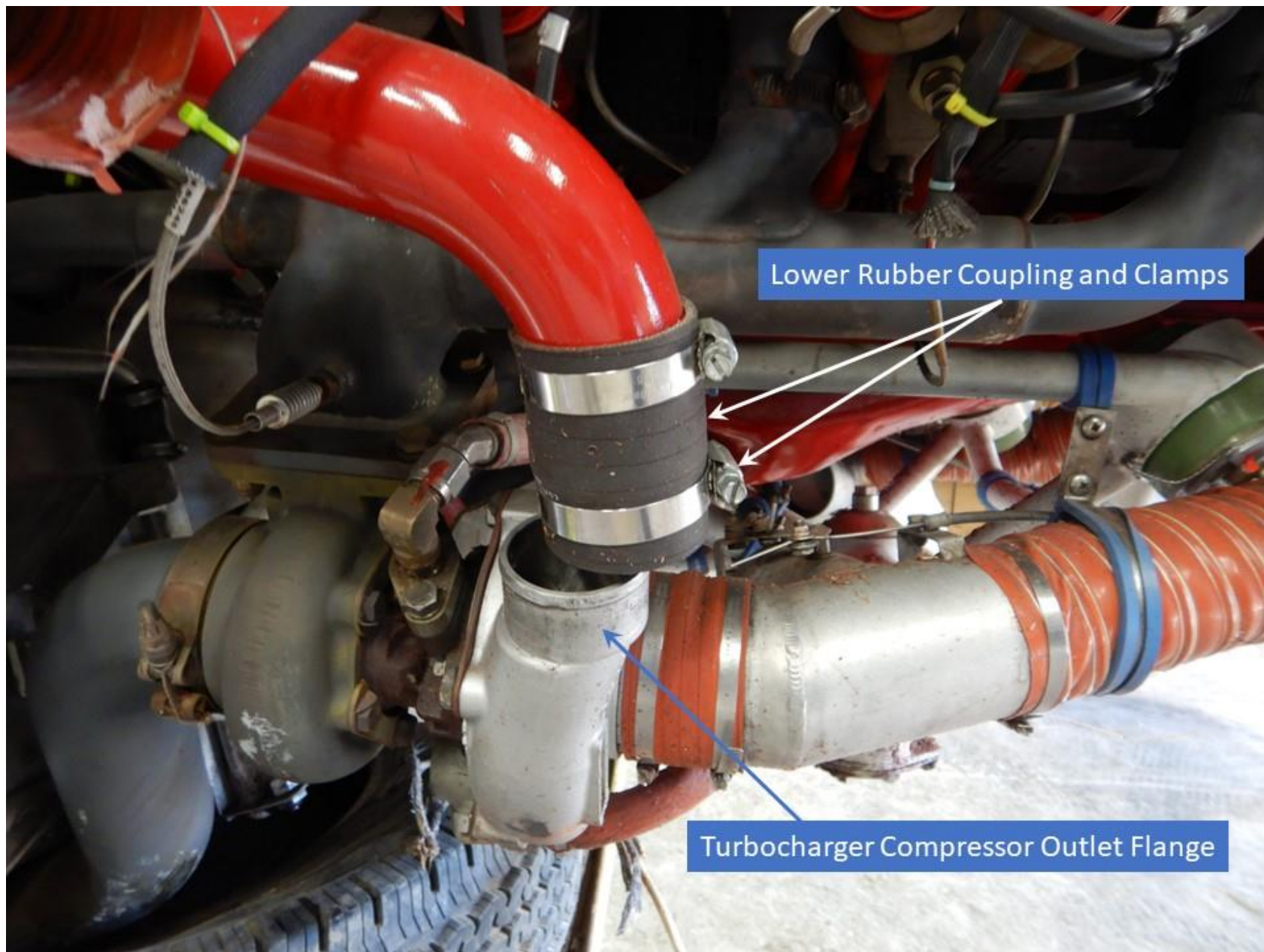
Photo 2 - Right side of engine and induction tube.
