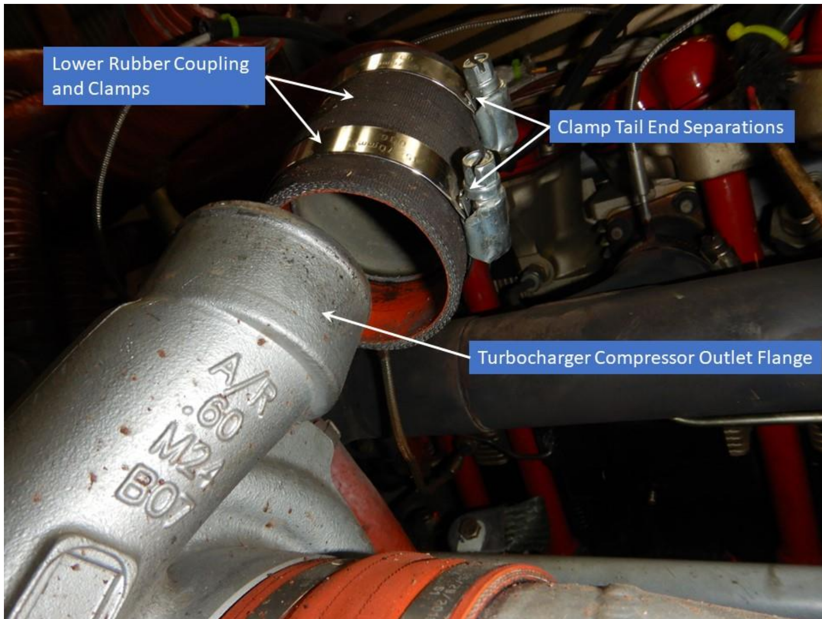
Photo 3 - Turbocharger and induction tube.
