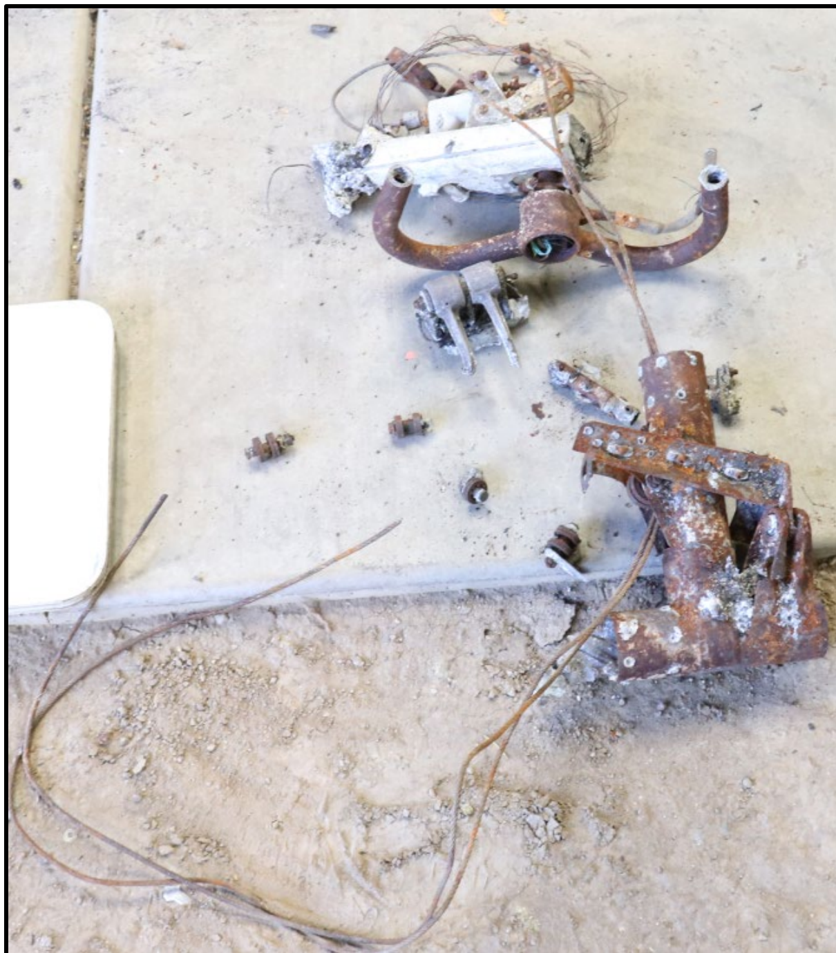
Figure 8: Right Control Column
