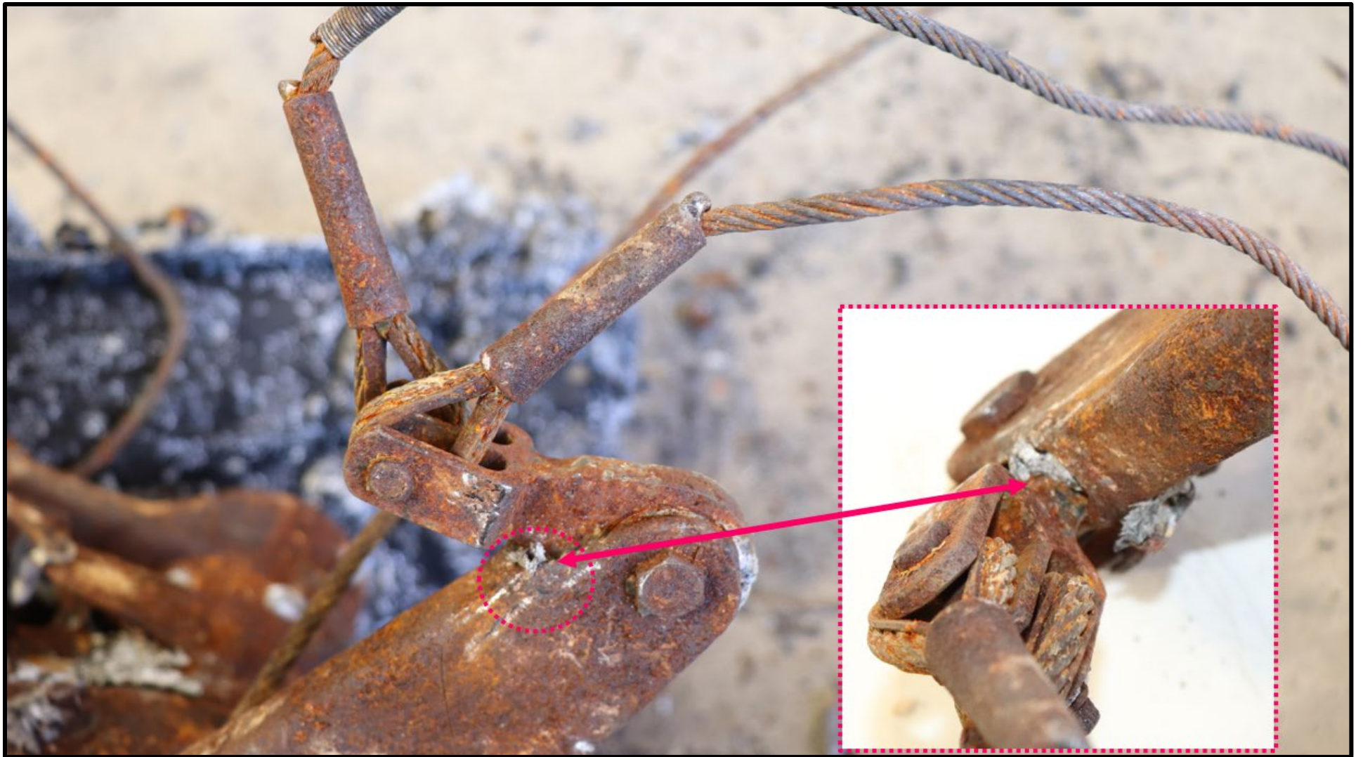
Figure 6: Forward Cable in Attach Point (Unknown Material Inside)
