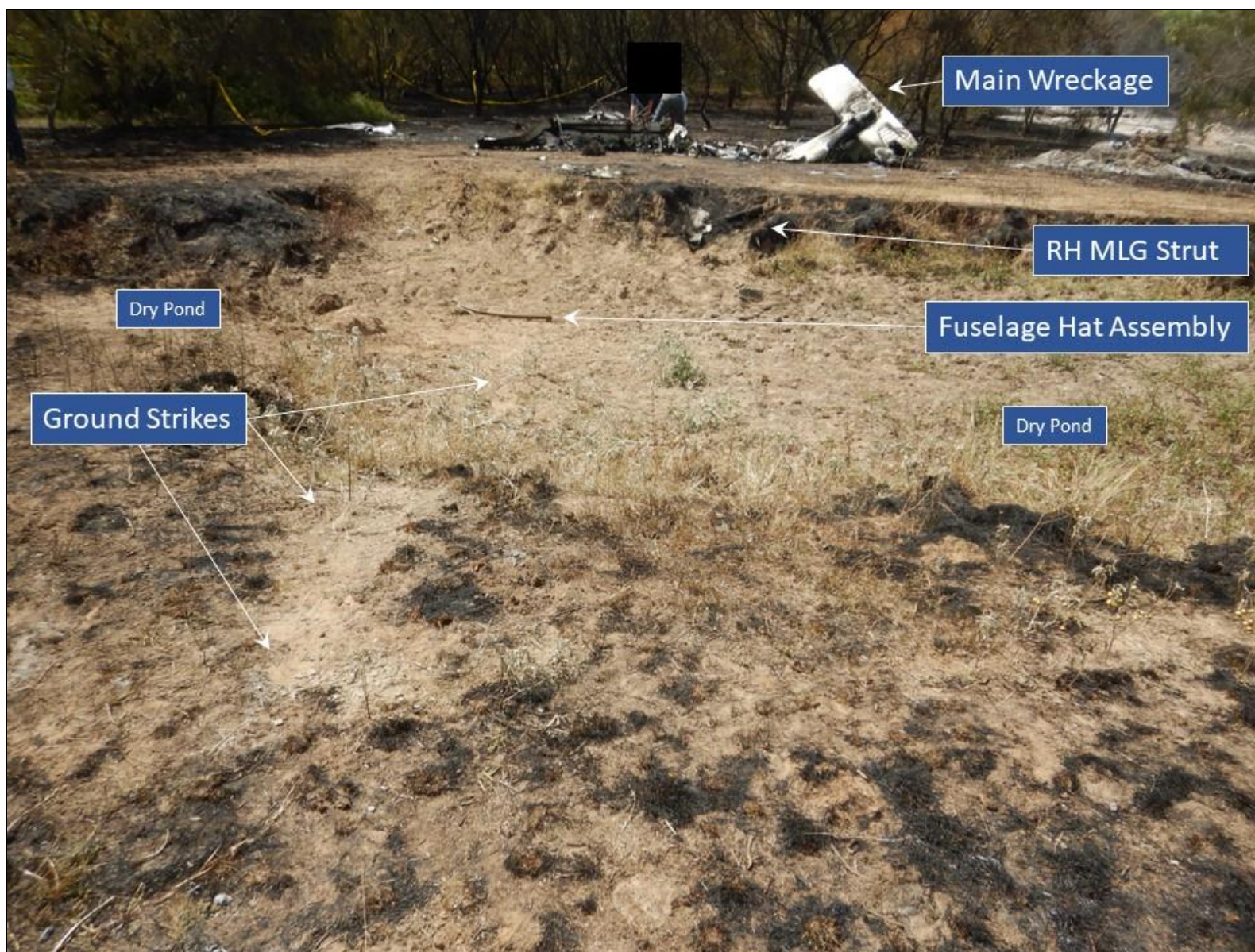
Photograph 2 - Accident site, ground scars and main wreckage.
