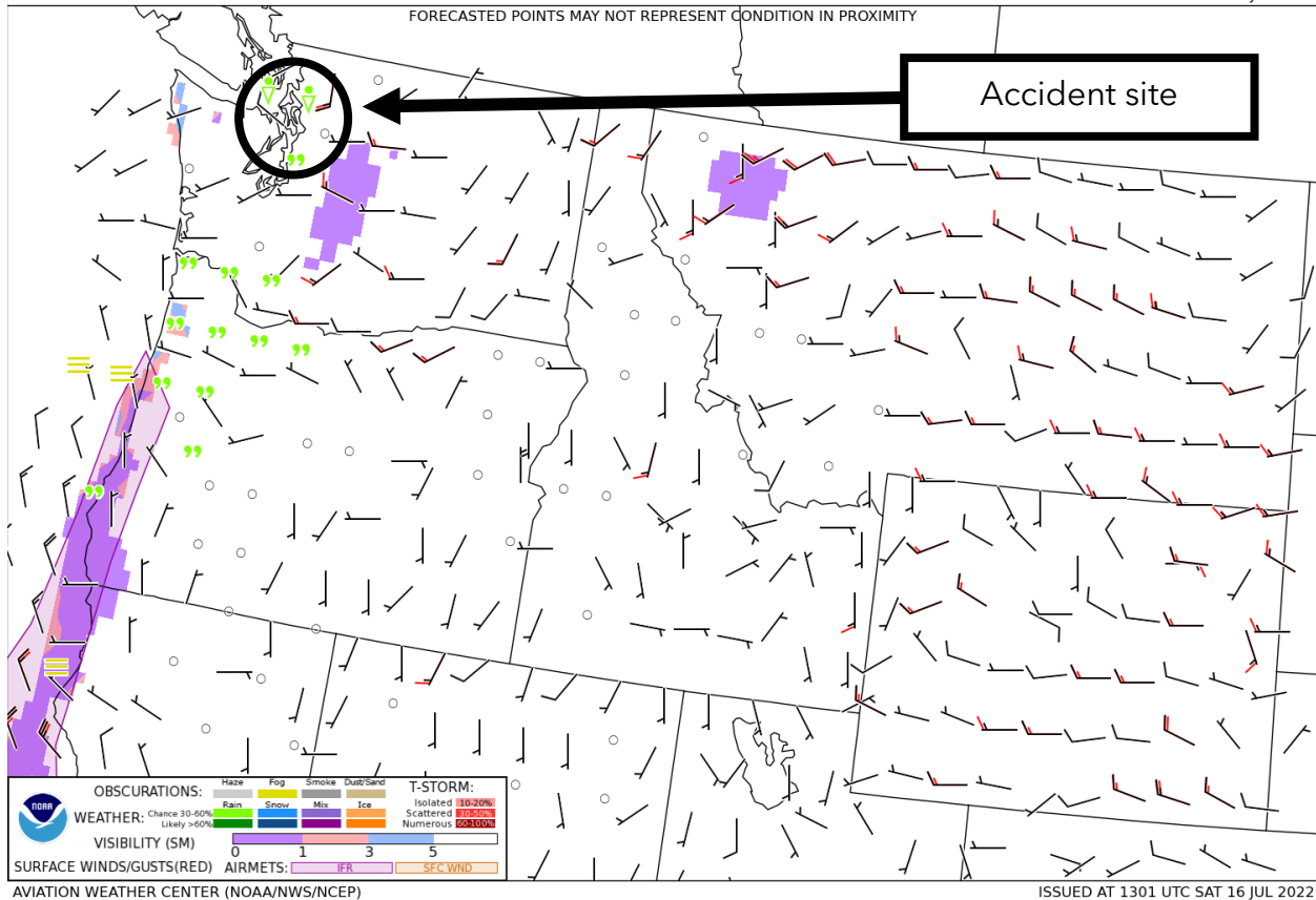
Figure 2. GFA Surface Forecast valid at 0800 PDT with forecast issued at 0601 PDT.
