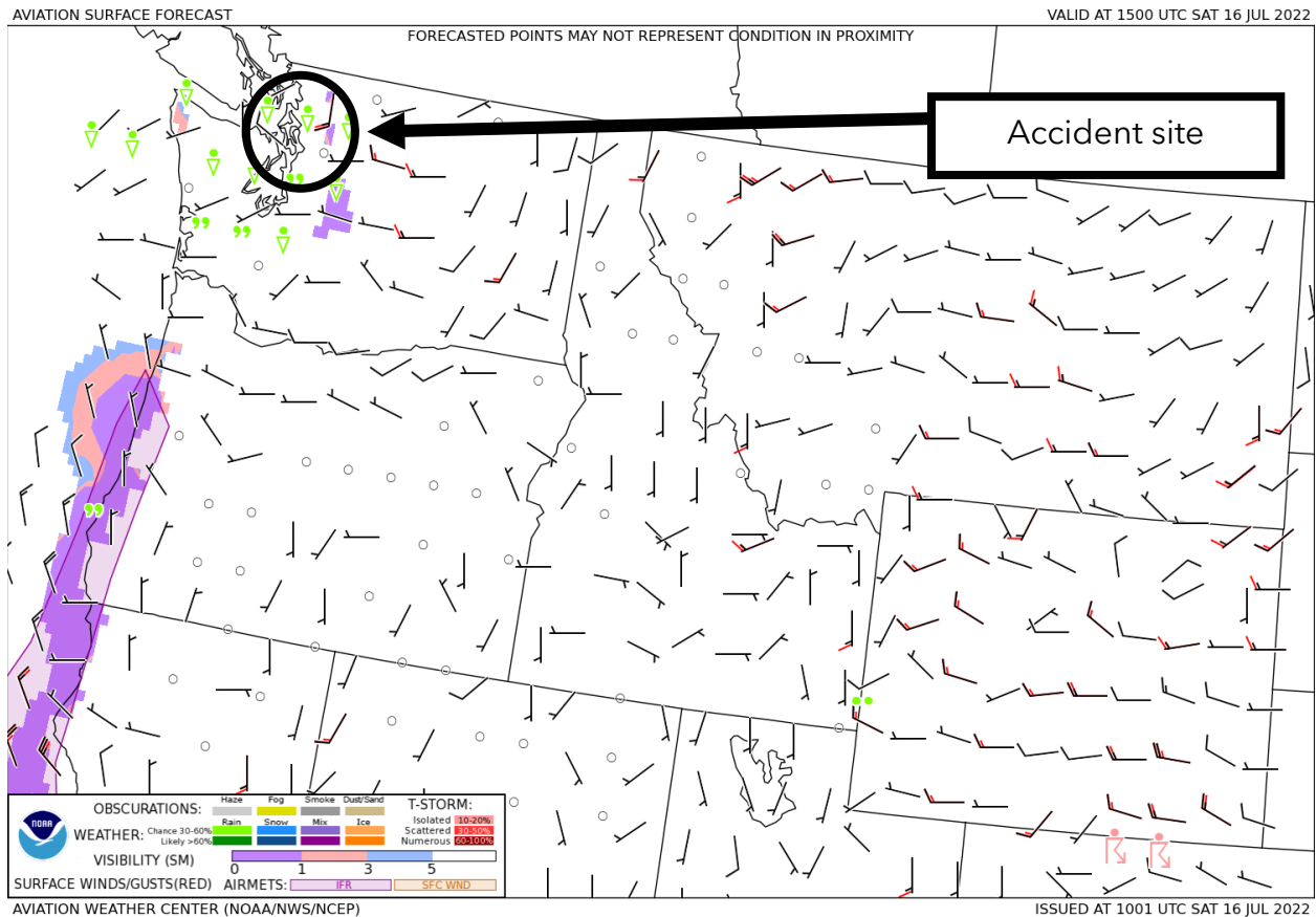
Figure 1. GFA Surface Forecast valid at 0800 PDT with forecast issued at 0301 PDT.
