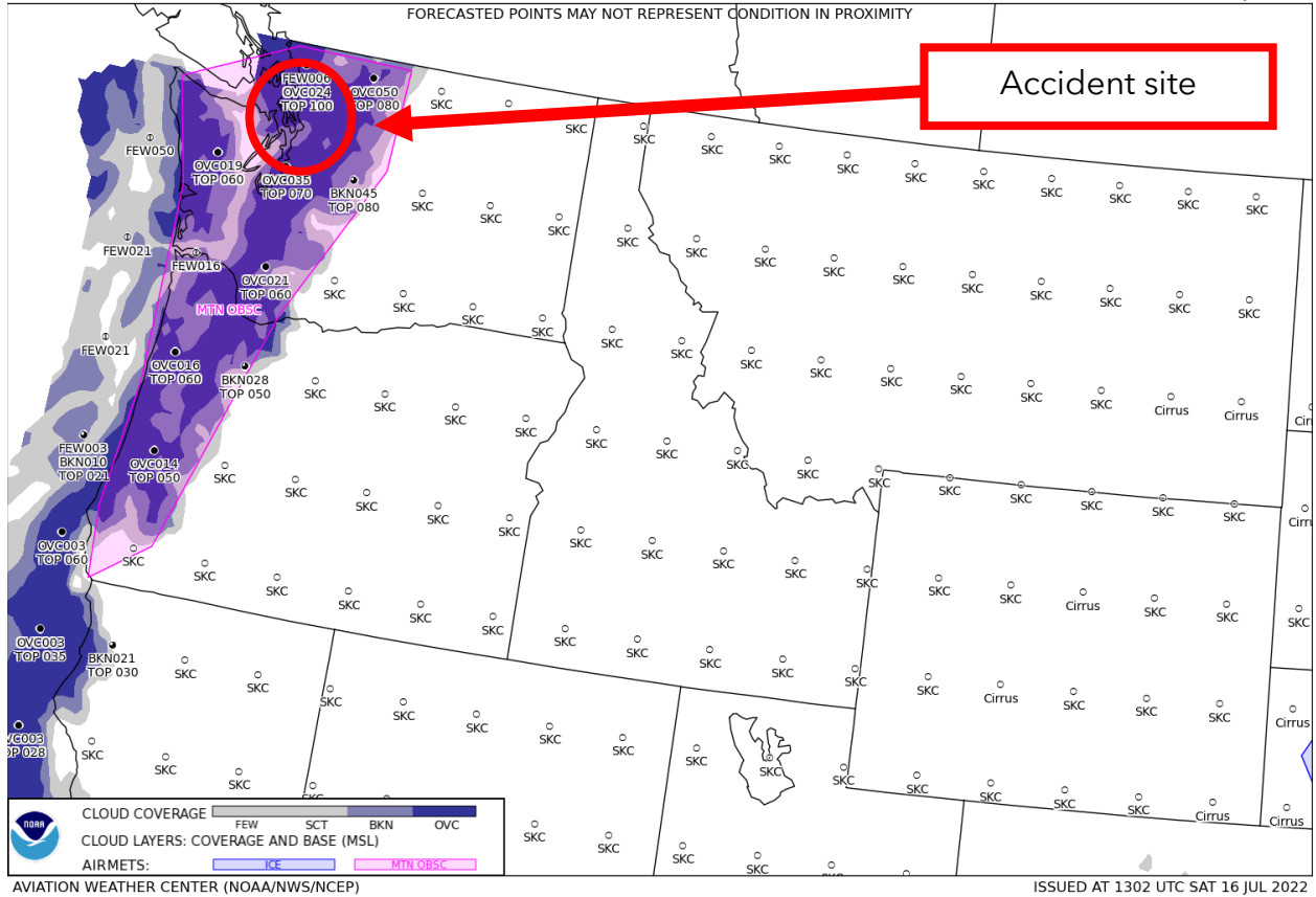
Figure 4. GFA Aviation Clouds Forecast valid at 0800 PDT with forecast issued at 0602 PDT.
