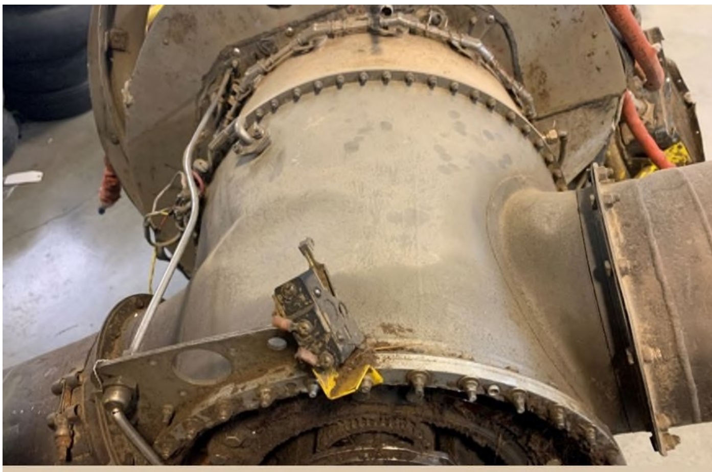
Photograph 2 - View of exhaust duct with external deformation consistent with torsional energy
