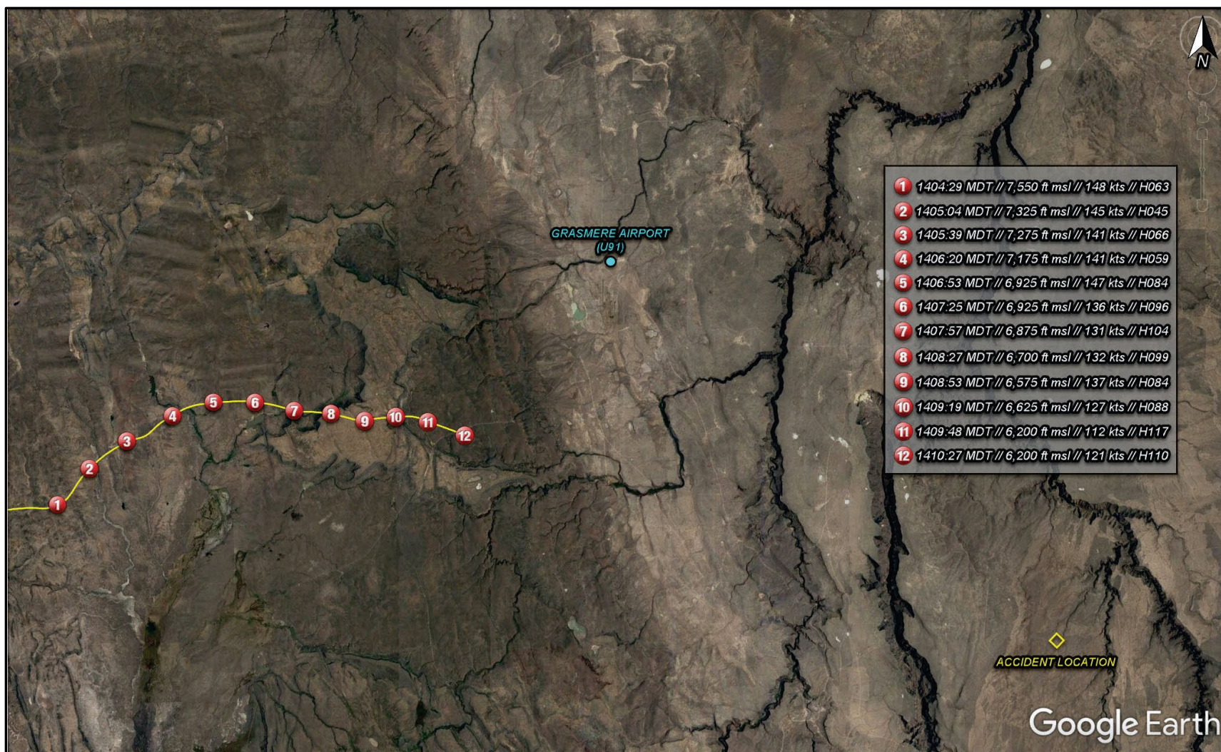
Figure 2 - Final segment of accident flight track with time, altitude, ground speed, and heading information.
