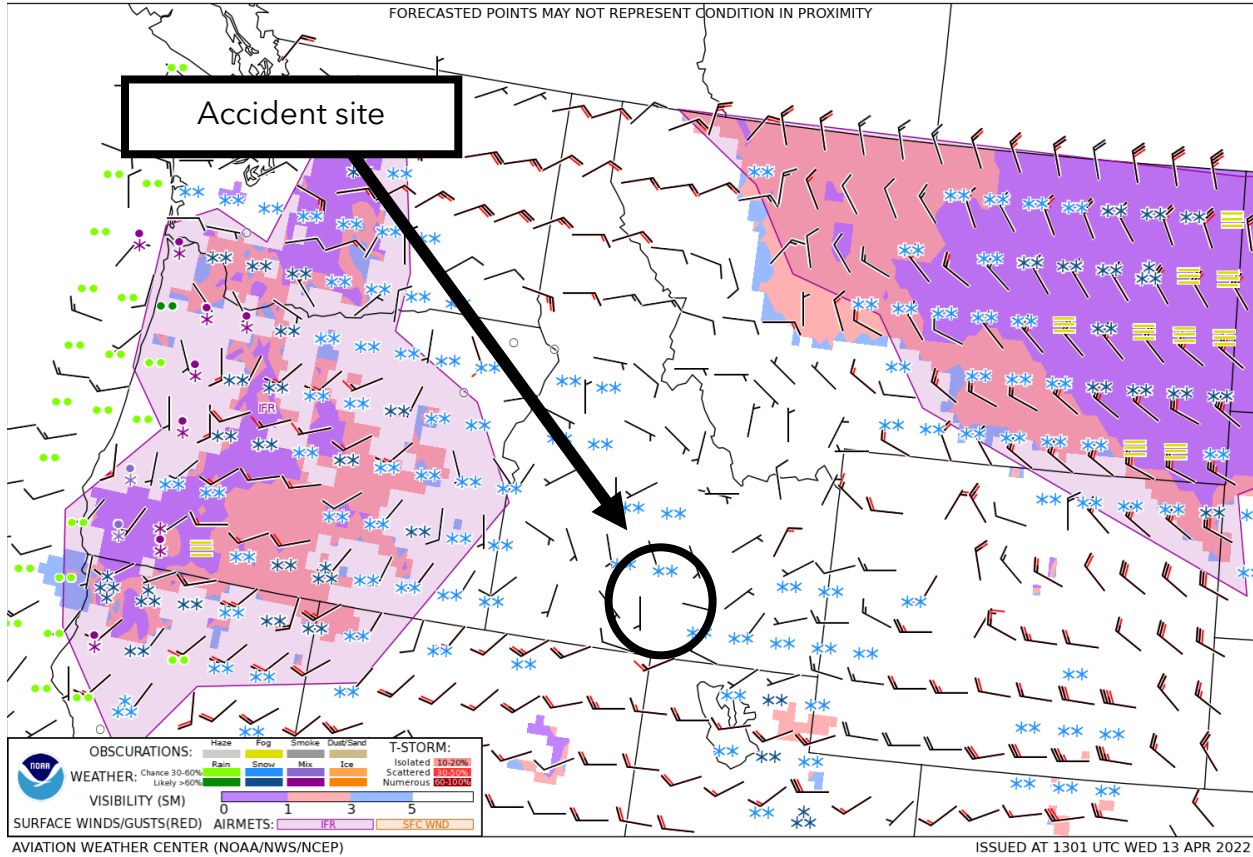
Figure 2. GFA Surface Forecast valid at 0900 MDT with forecast issued at 0701 MDT.
