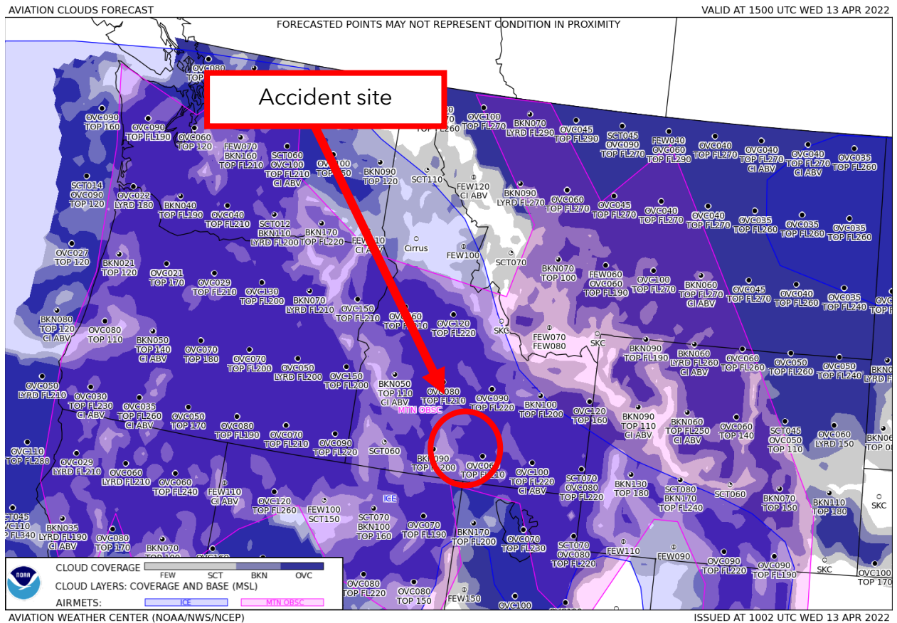
Figure 3. GFA Aviation Clouds Forecast valid at 0900 MDT with forecast issued at 0402 MDT.
