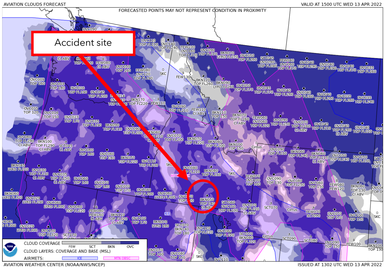
Figure 4. GFA Aviation Clouds Forecast valid at 0900 MDT with forecast issued at 0702 MDT.
