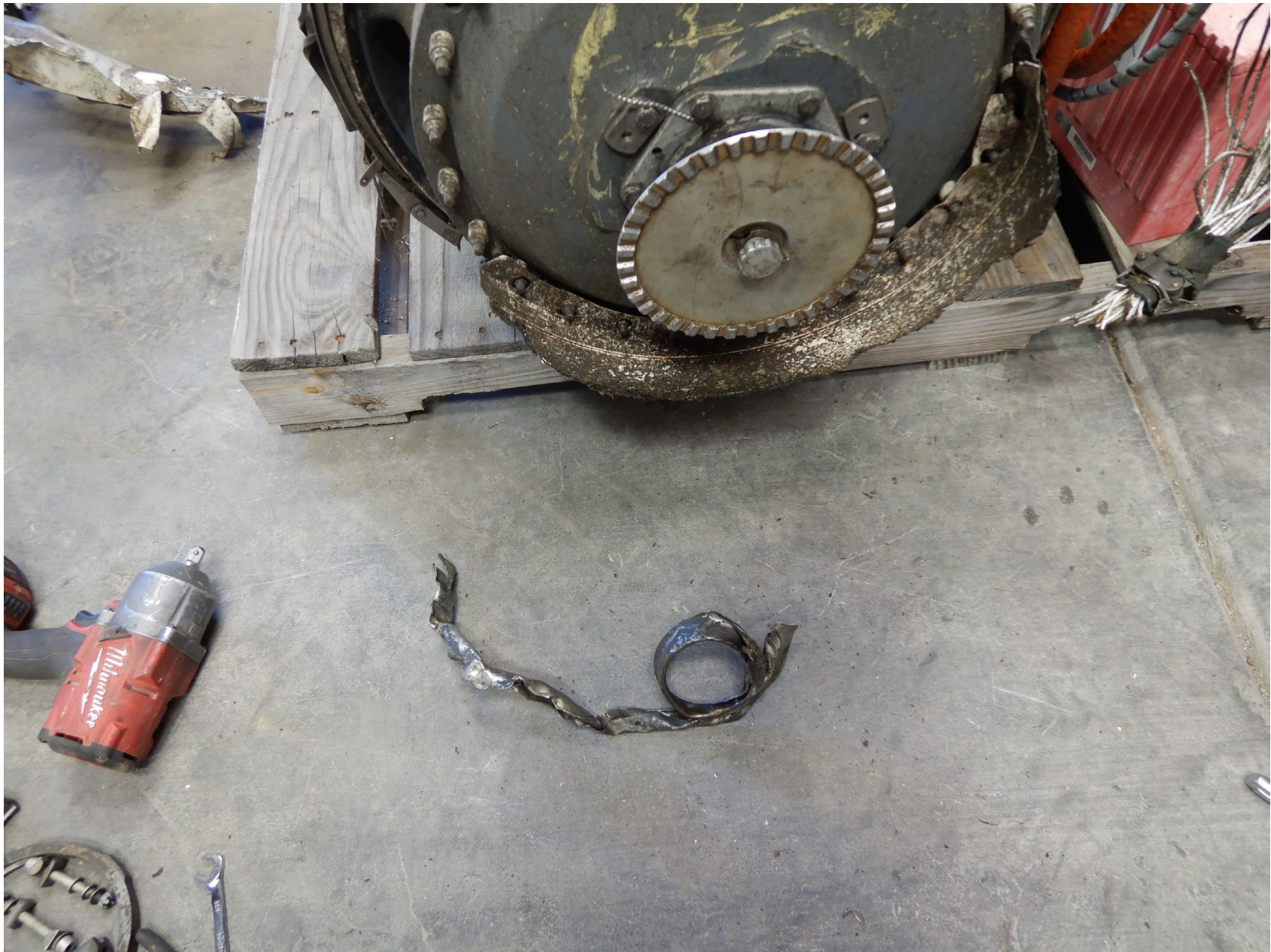
Photo 10 – Engine output shaft and a section of fire wall that wrapped around the output shaft.
