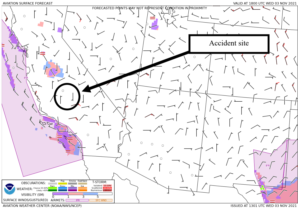
Figure 1 – GFA Surface Forecast valid at 1100 PDT with forecast issued at 0601 PDT.
