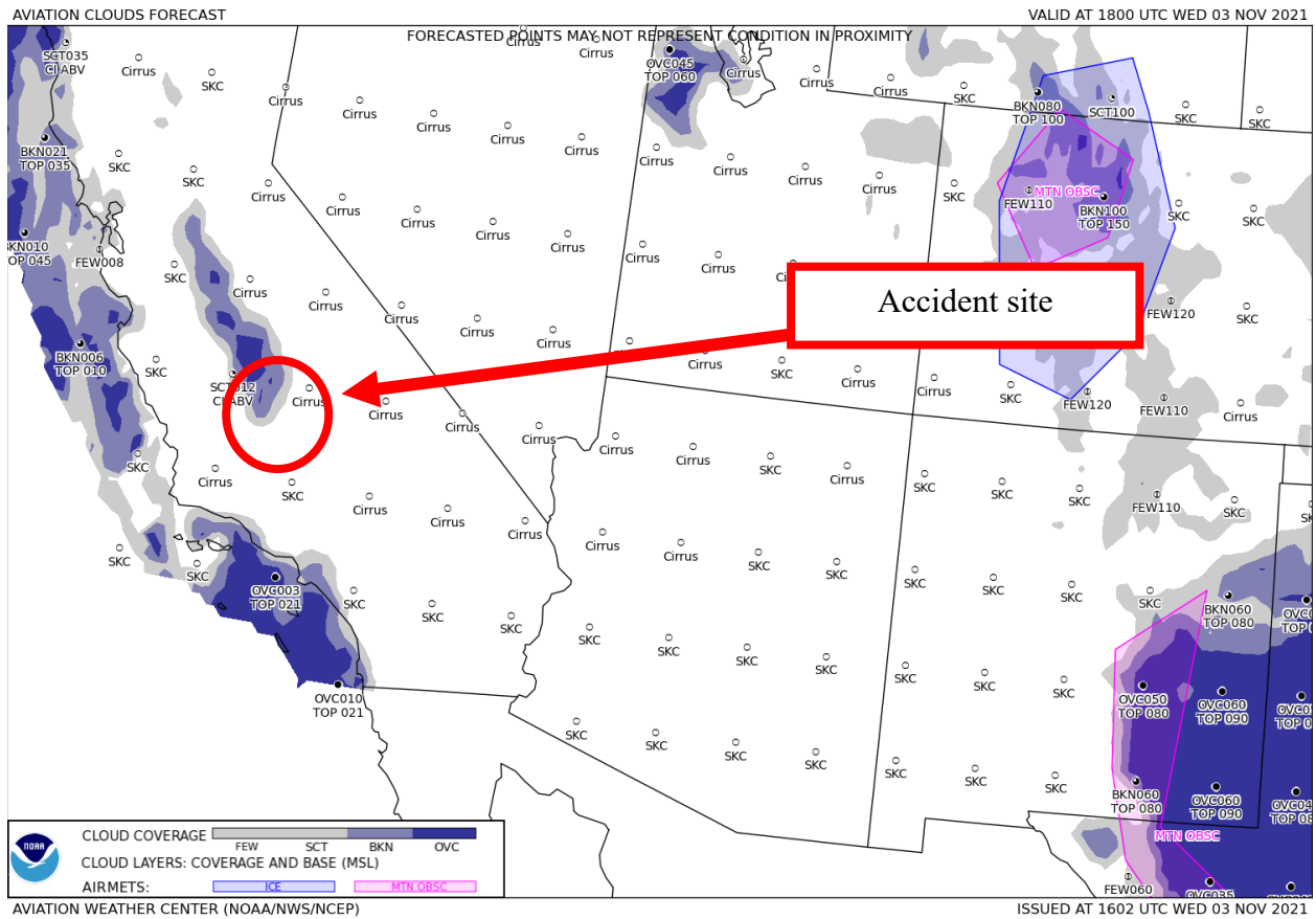
Figure 4 – GFA Aviation Clouds Forecast valid at 1100 PDT with forecast issued at 0902 PDT.
