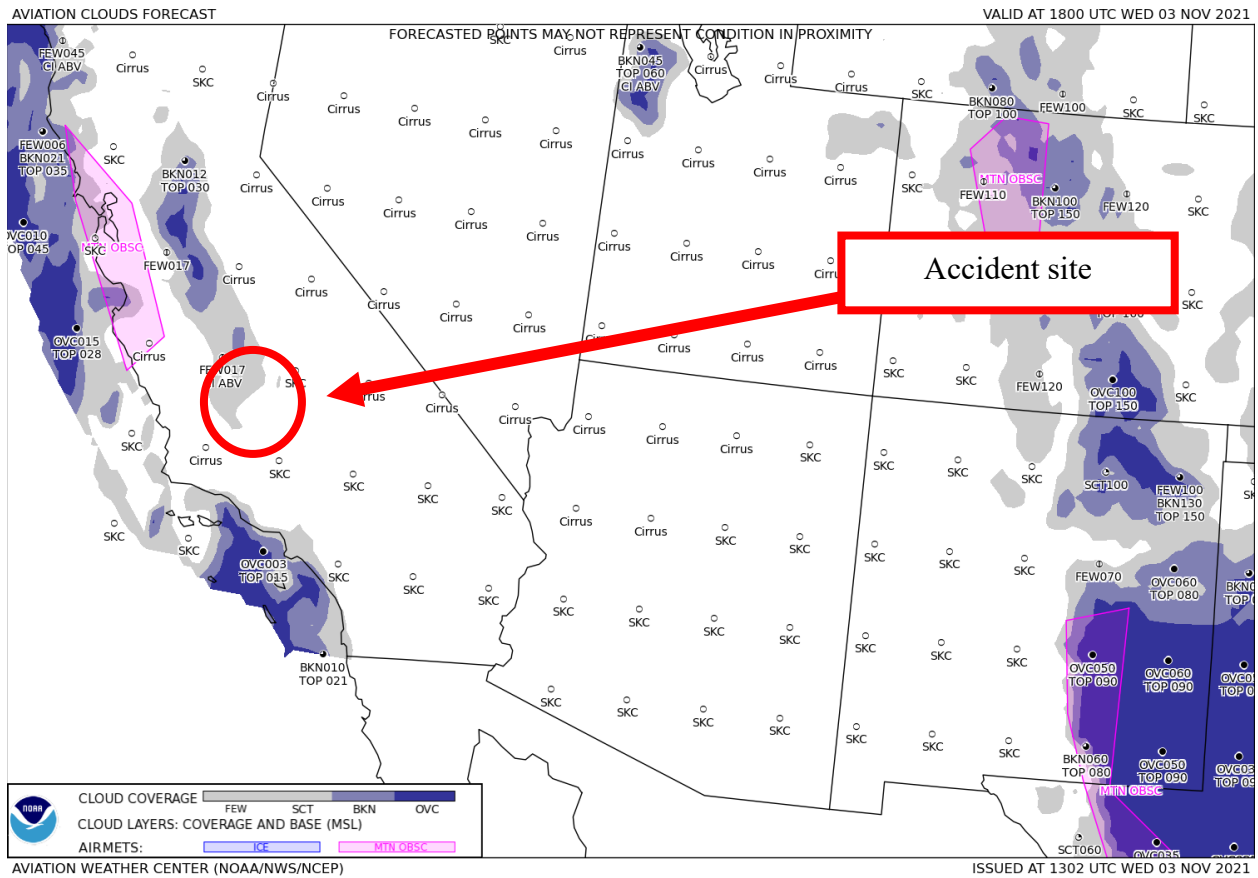
Figure 3 – GFA Aviation Clouds Forecast valid at 1100 PDT with forecast issued at 0602 PDT.
