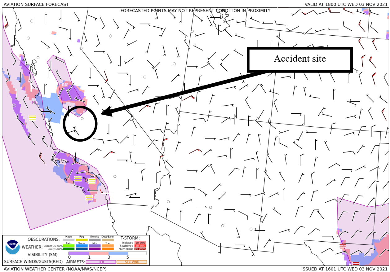
Figure 2 – GFA Surface Forecast valid at 1100 PDT with forecast issued at 0901 PDT.
