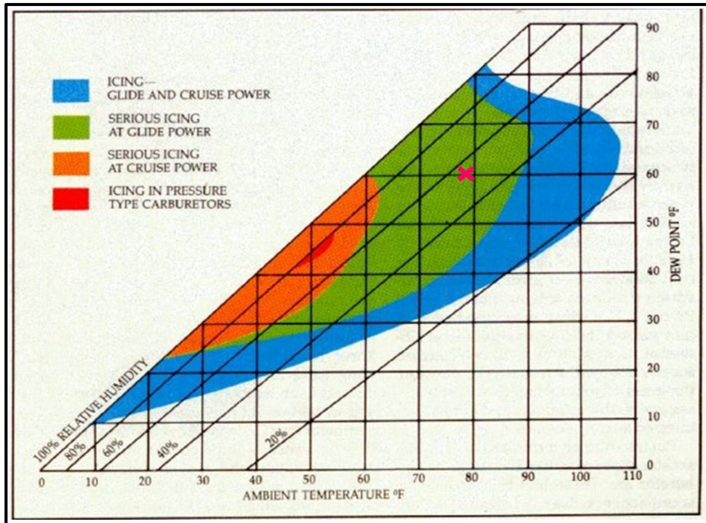
Figure 1: FAA Carburetor Icing Probability Chart
