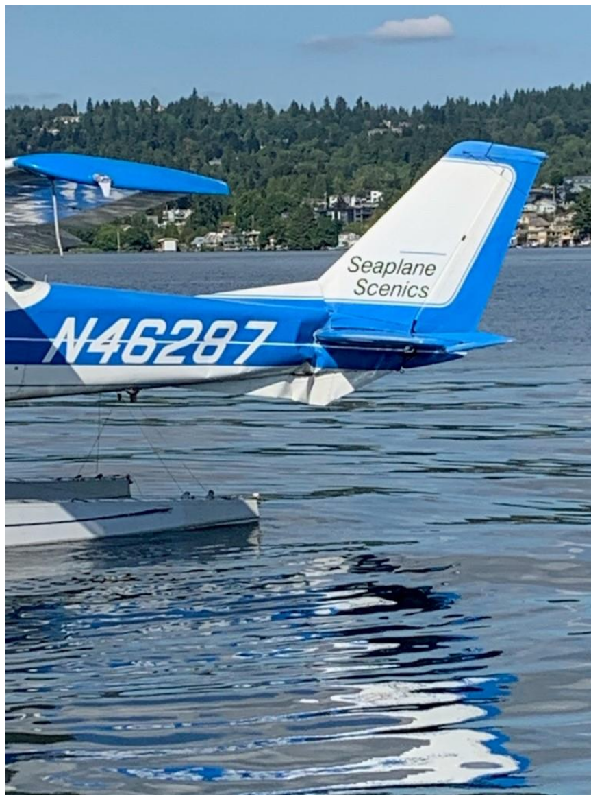
Photo 1 – View of damage to the floatplane’s tail section (Courtesy of FAA)
