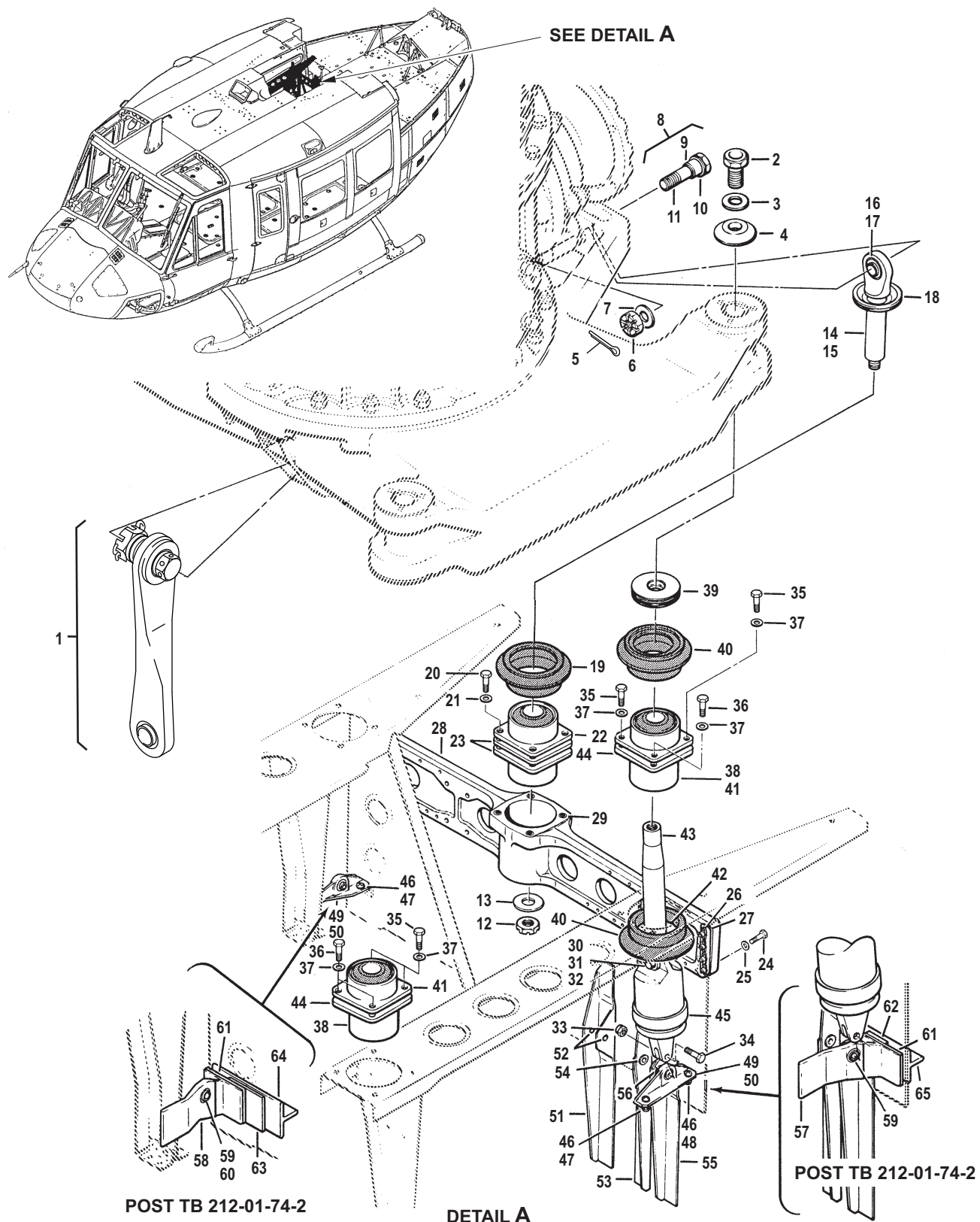
Figure 63-25. Pylon Support Installation
