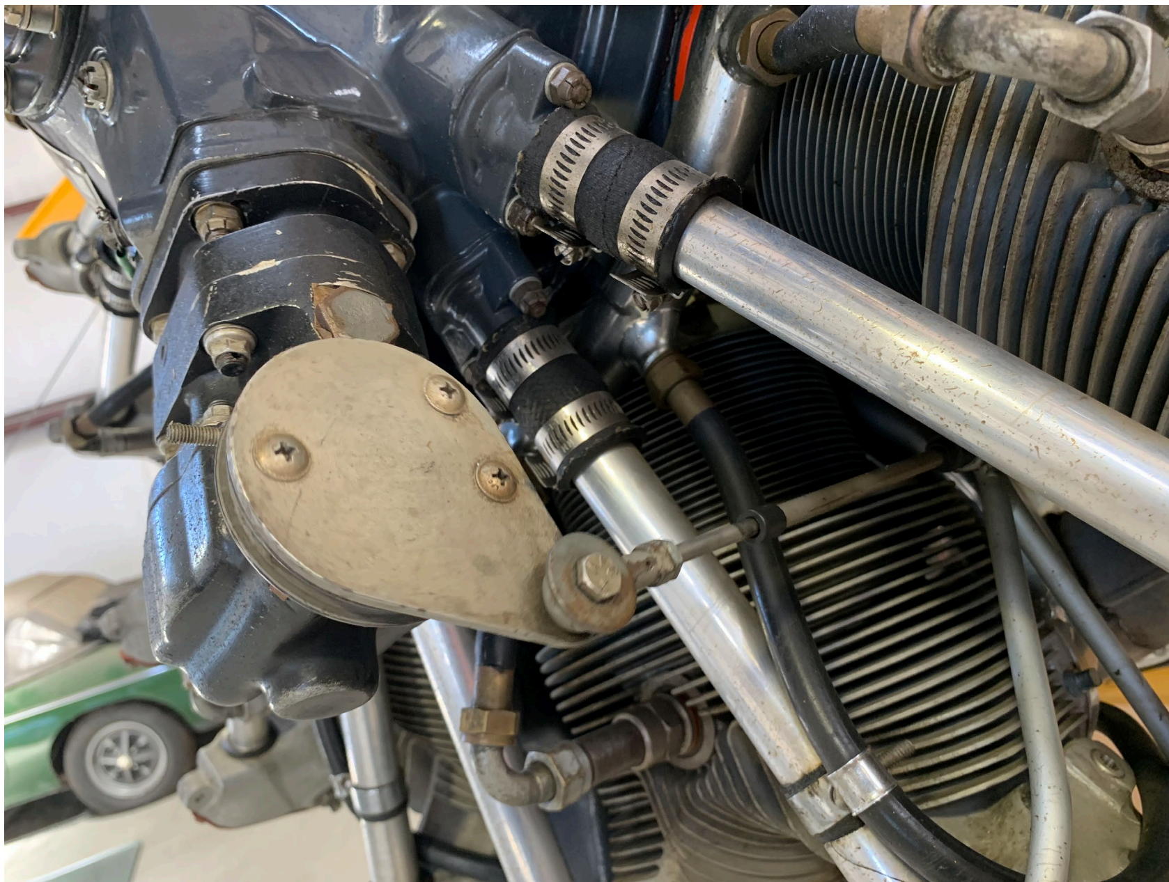
Photo 7 – View of Propeller Governor installed on accident engine (photo courtesy of FAA)
