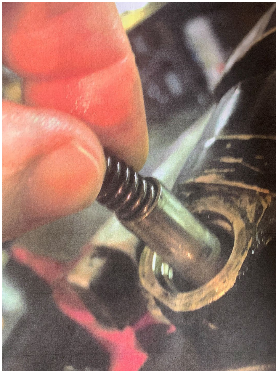
Photo 5 – View of relief valve spring removed from relief valve plunger (courtesy of Wings West Exchange & Overhaul, Inc)
