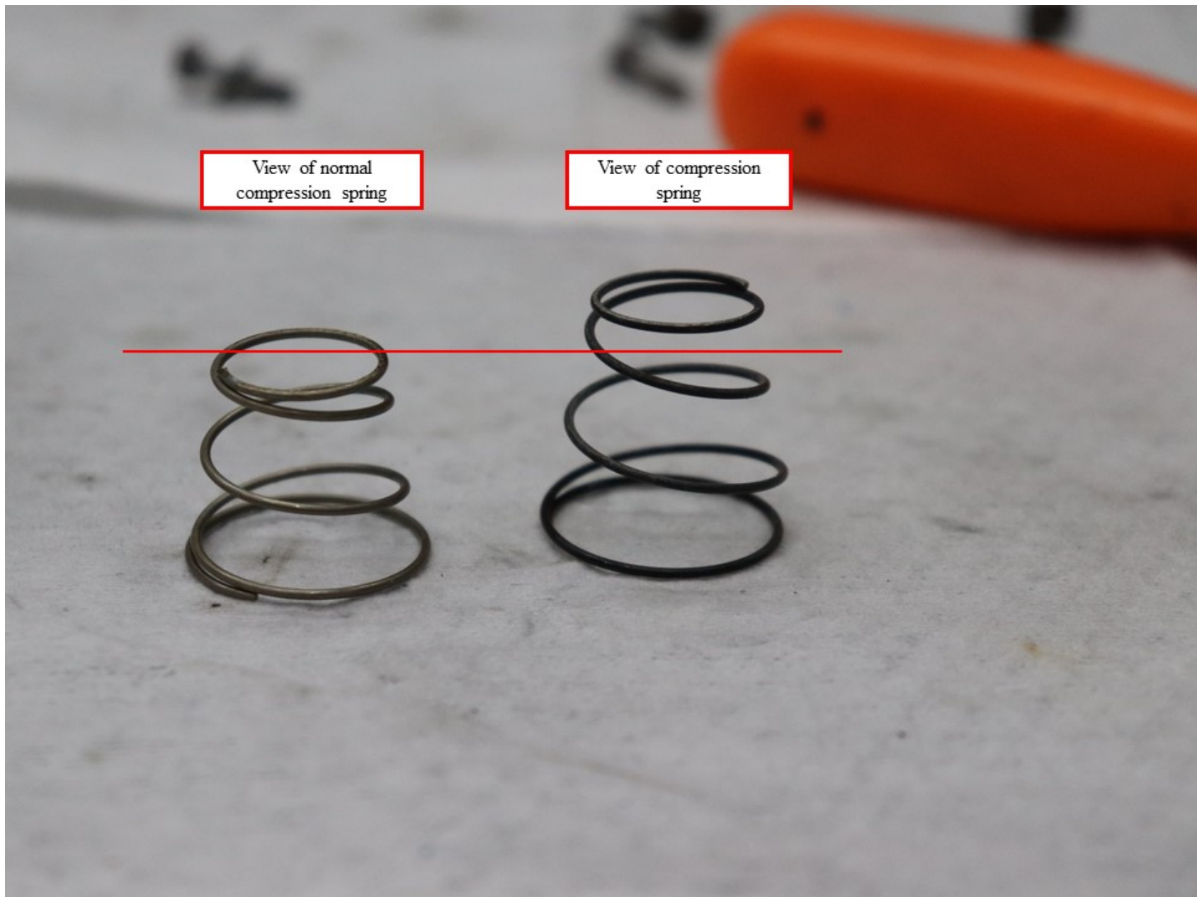
Photo 6 - View of fuel flow manifold valve compression spring comparison (photo courtesy of the NTSB)
