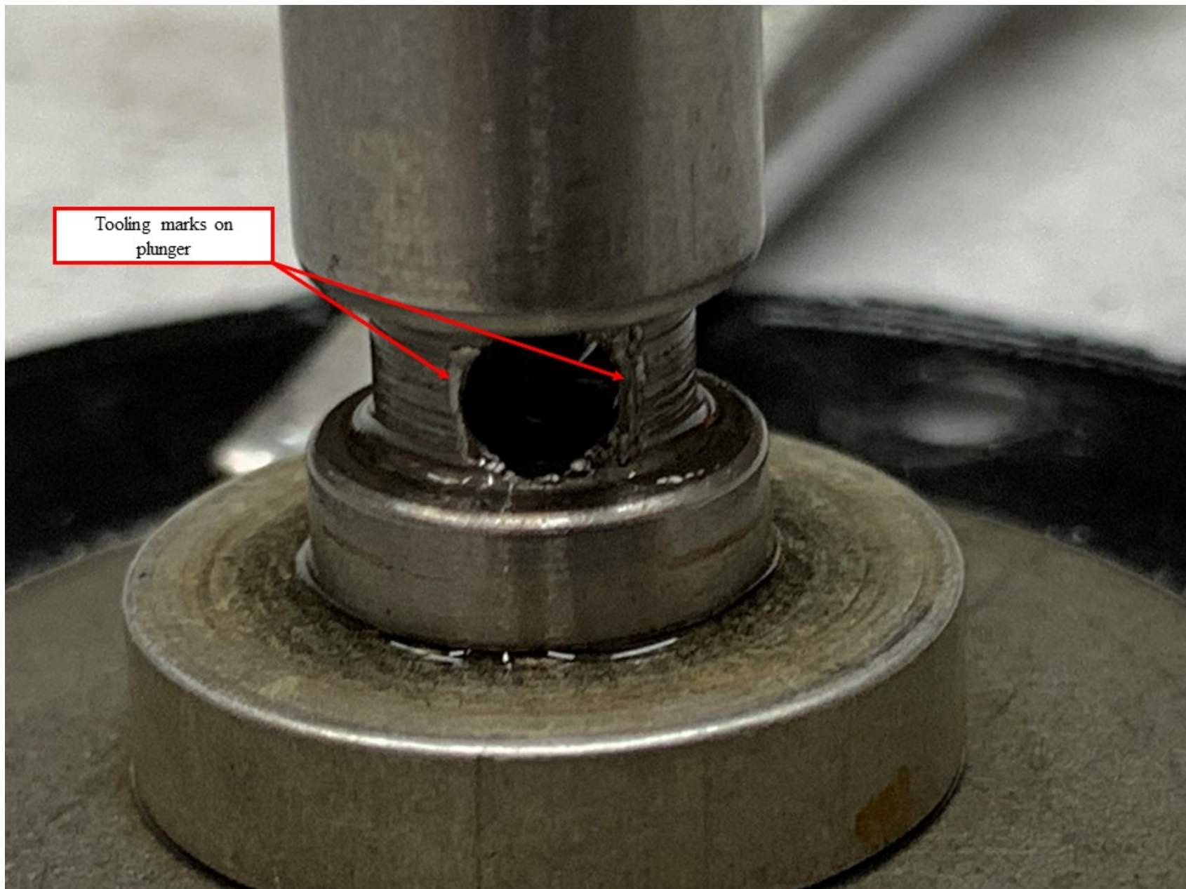
Photo 5 - View of tooling marks on fuel flow manifold valve plunger (photo courtesy of the NTSB)
