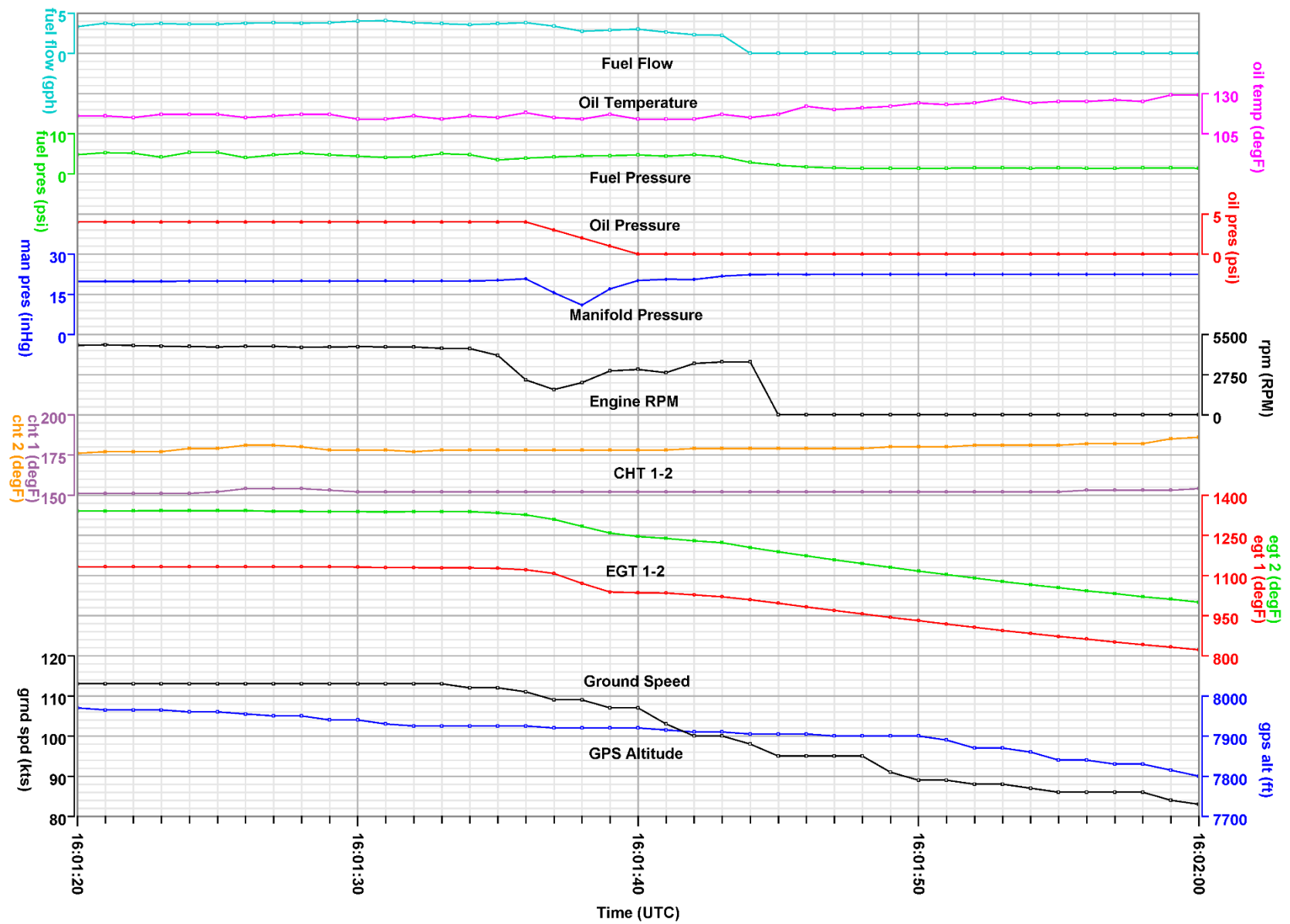
Plot of Dynon EMS-D120 parameters between 16:01:20 and 16:02:00 UTC.
