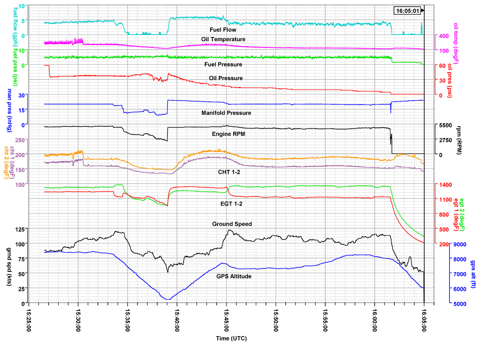
Plot of Dynon EMS-D120 parameters for the entire event session.
