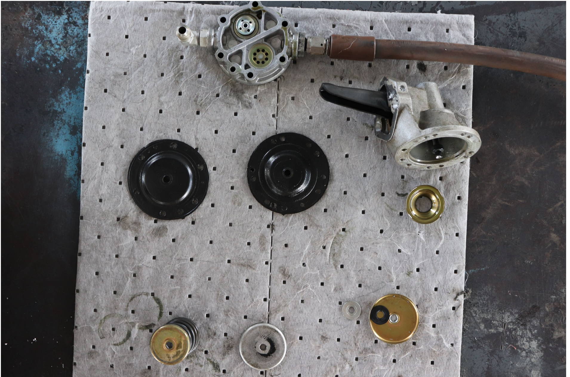
Photo 8 - View of engine driven fuel pump during exam (photo courtesy of the NTSB)
