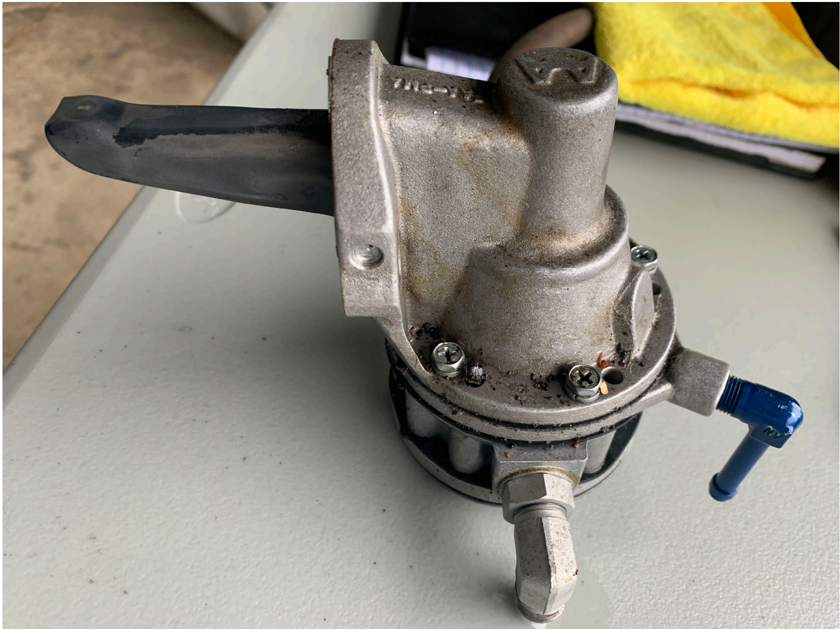
Photo 7 - View of engine driven fuel pump during exam (photo courtesy of the NTSB)
