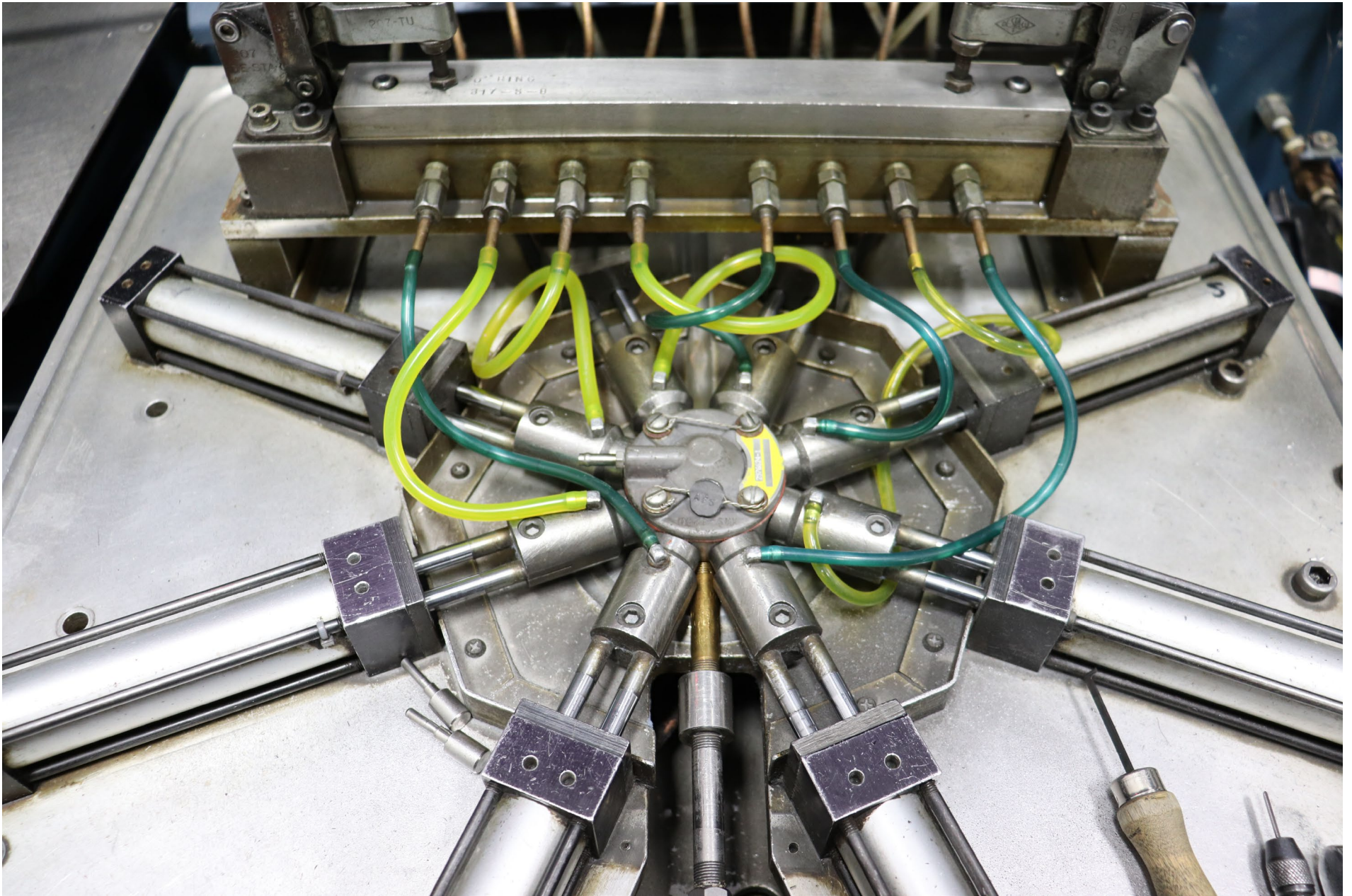
Photo 6 - View of fuel flow divider during exam (photo courtesy of the NTSB)
