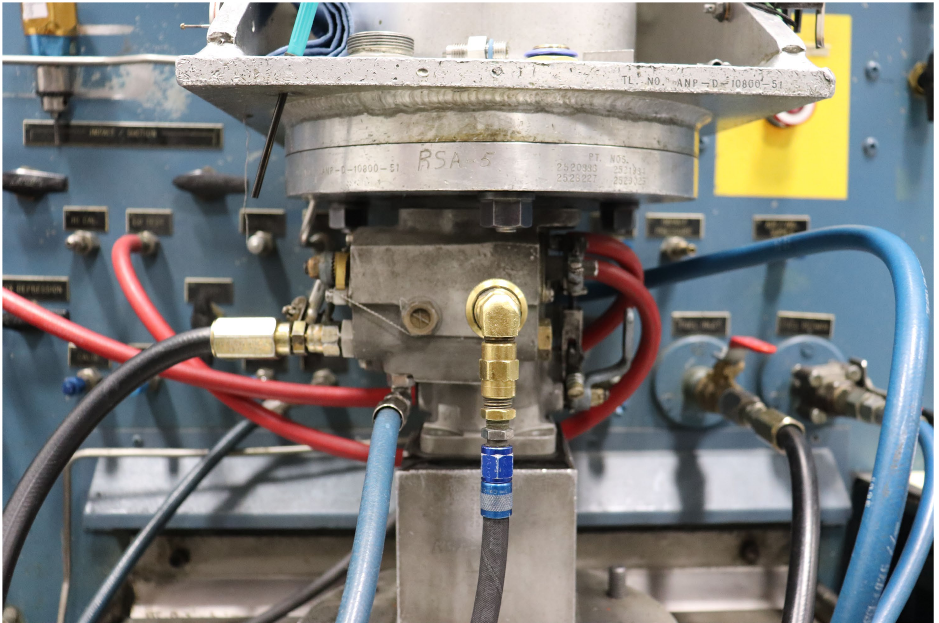
Photo 5 - View of fuel servo during exam (photo courtesy of the NTSB)
