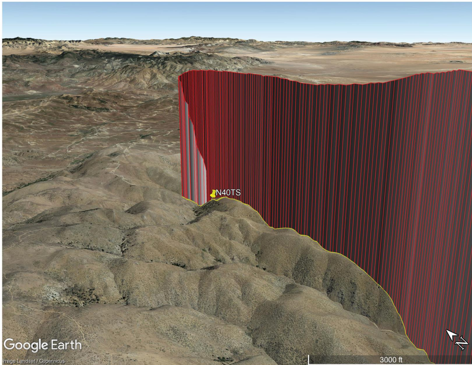
Photo 4 – Accident flight track and accident site location.
