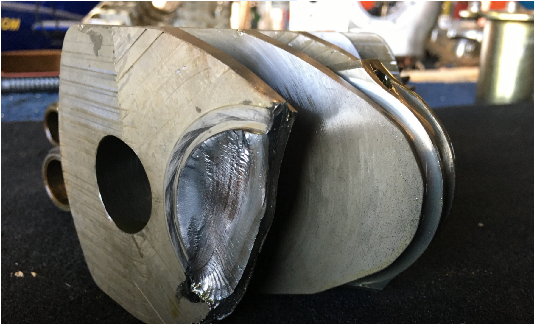
Photo 9 - N975G Broken Crankshaft, courtesy FAA FSDO
