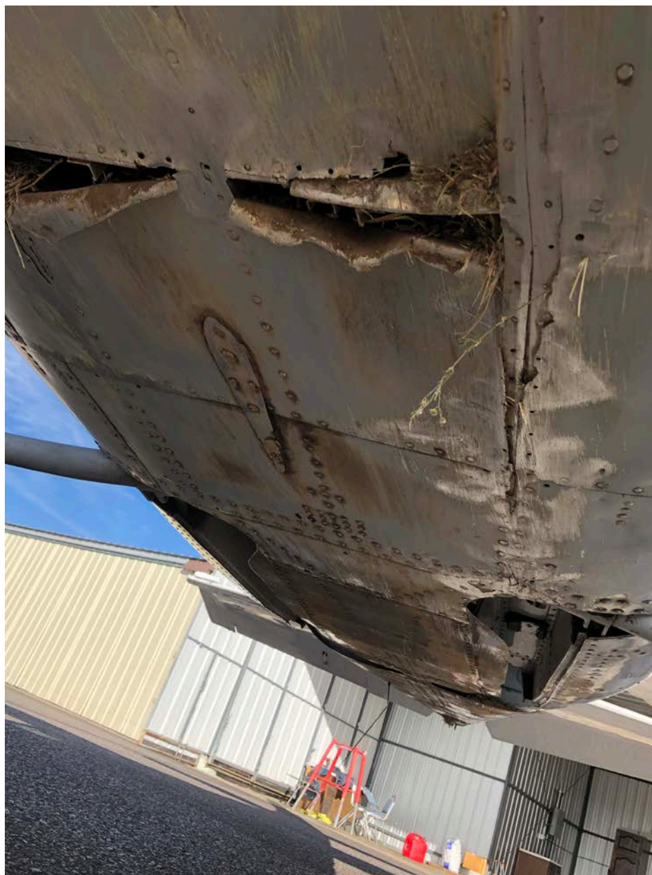
Photo 1 – View of Undercarriage (RHeineman)
