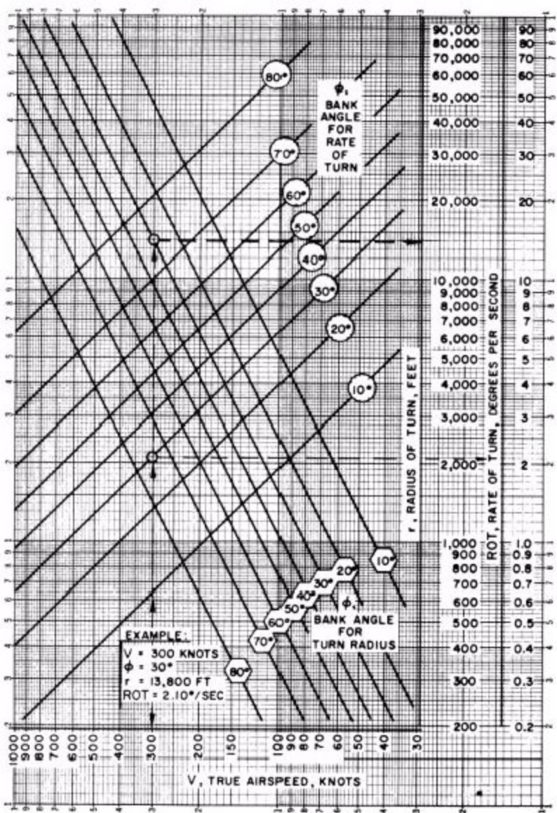
Figure 2.29. General Turn Performance (Constant Altitude. Steady Turn)
