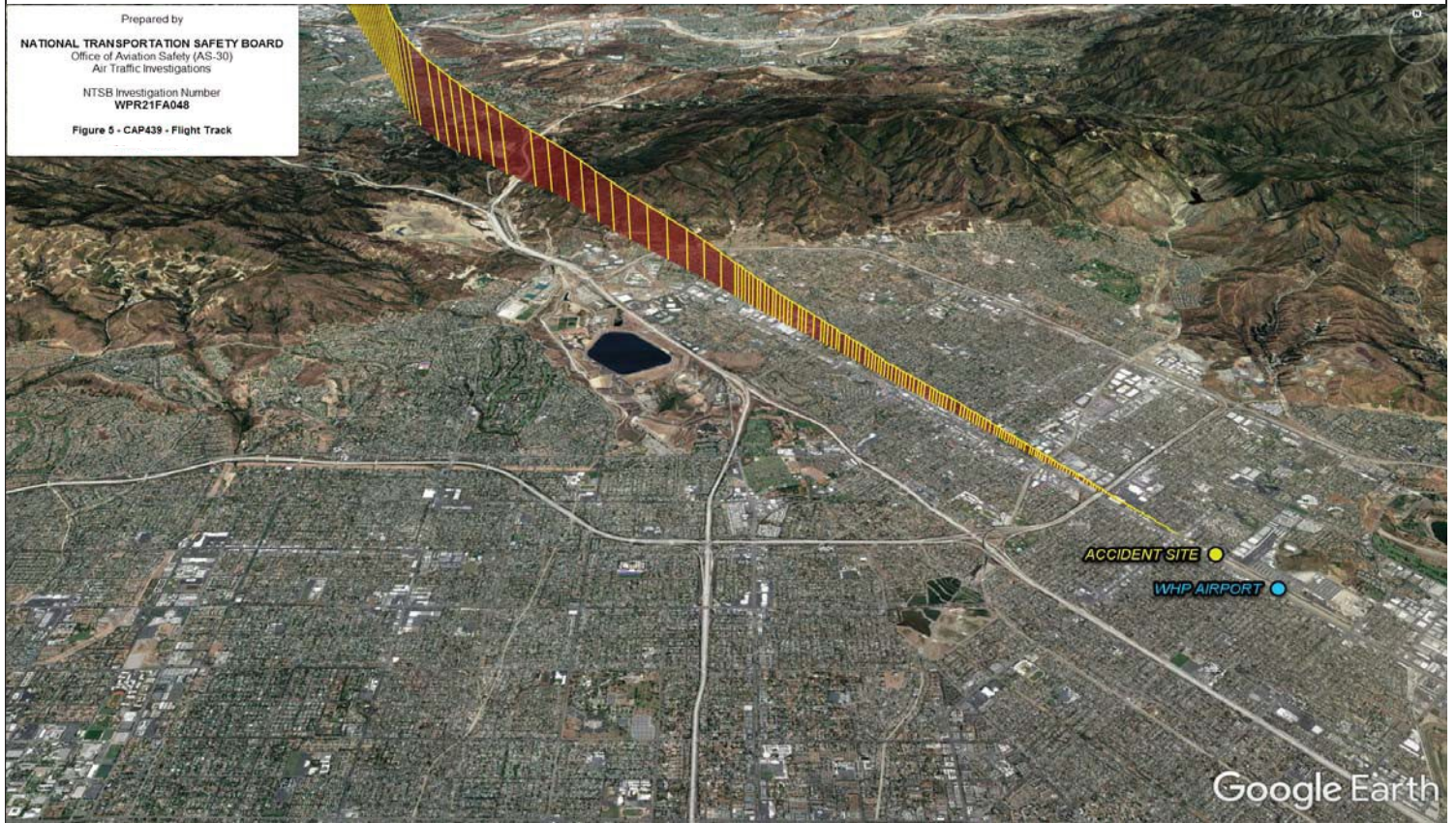
Caption Final segment of the accident flight track in profile view.
