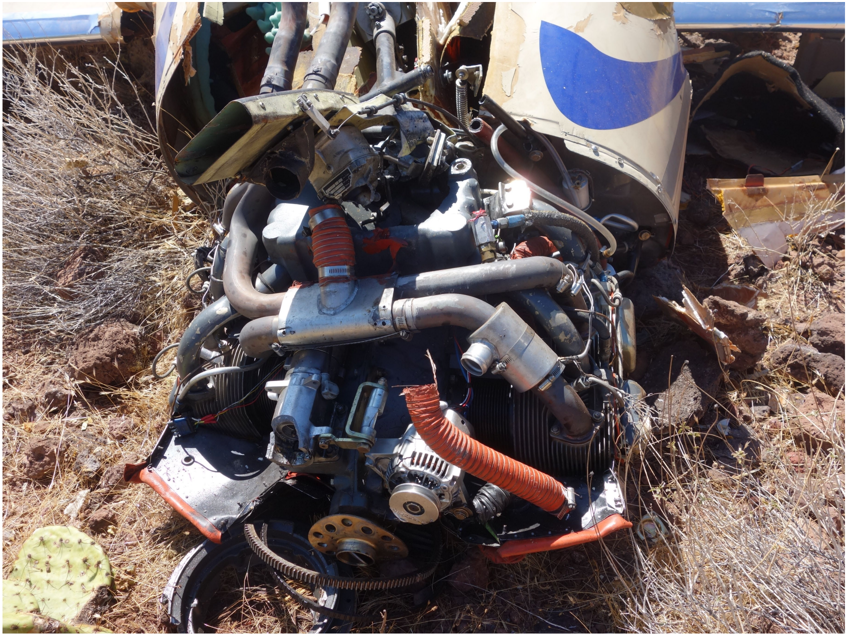
Photo 2 – View of the engine at the accident site.
