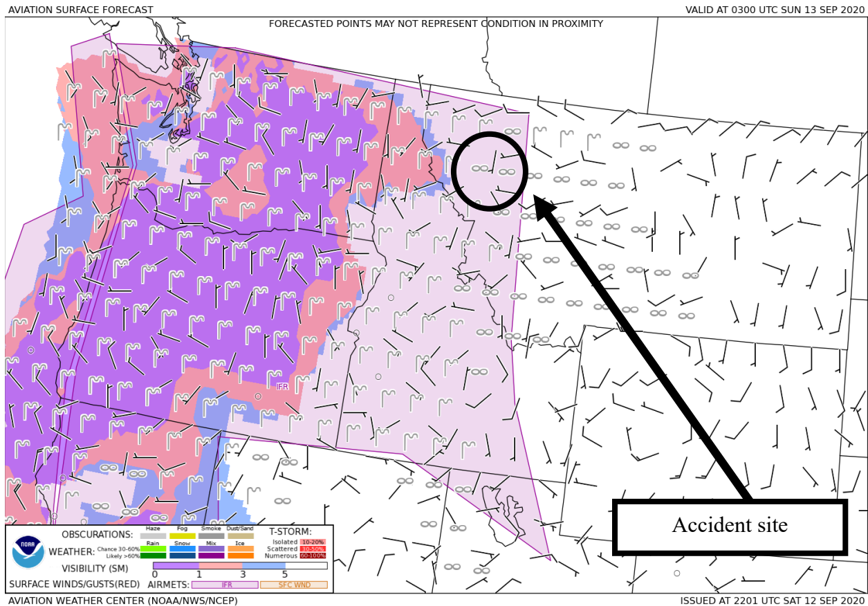
Figure 1 – GFA Surface Forecast valid at 2100 MDT with forecast issued at 1601 MDT
