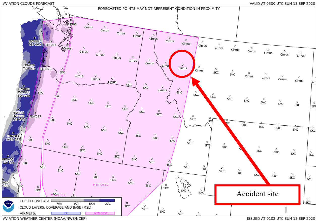
Figure 4 – GFA Aviation Clouds Forecast valid at 2100 MDT with forecast issued at 1902 MDT
