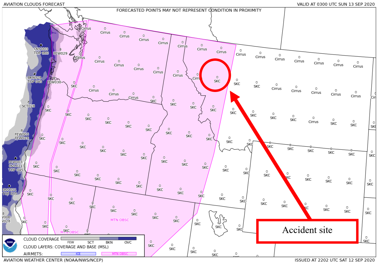
Figure 3 – GFA Aviation Clouds Forecast valid at 2100 MDT with forecast issued at 1602 MDT
