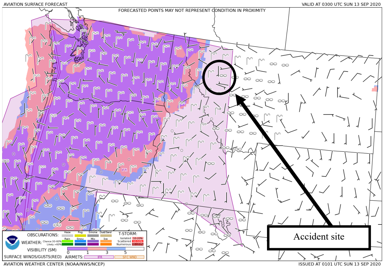
Figure 2 – GFA Surface Forecast valid at 2100 MDT with forecast issued at 1901 MDT
