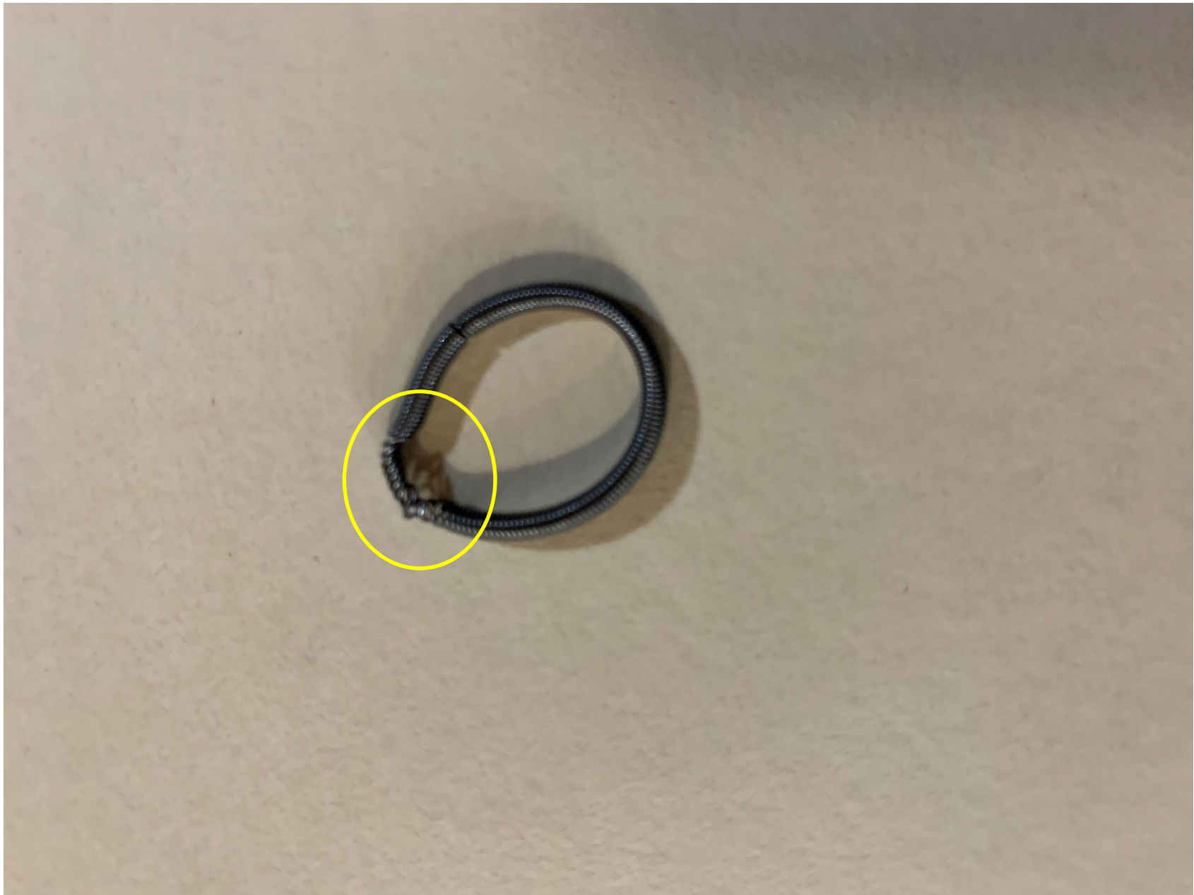
Photo 5 - View of mechanical hydraulic pump load spring damage (photo courtesy of the maintenance facility)
