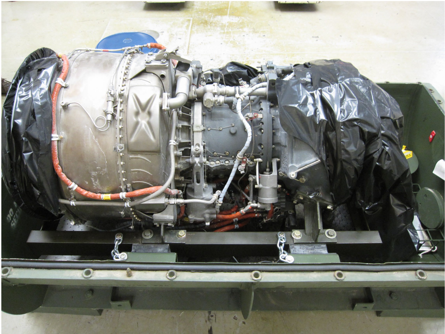
Photo 6 – Engine, right view. Photo Operator.
