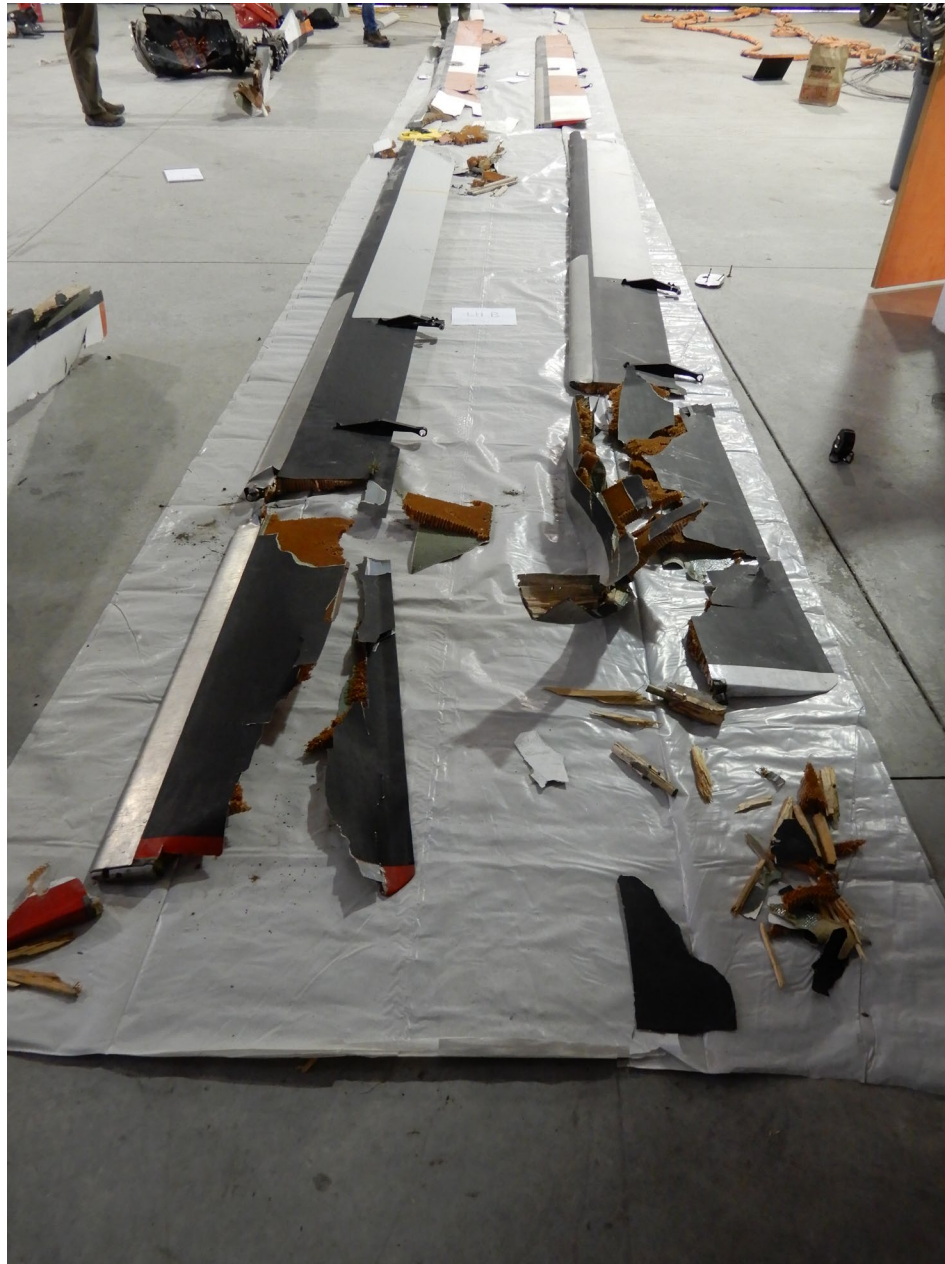
Photo 9 – Left-side rotor blades. Red blade is on the left, and the white blade in on the right.
