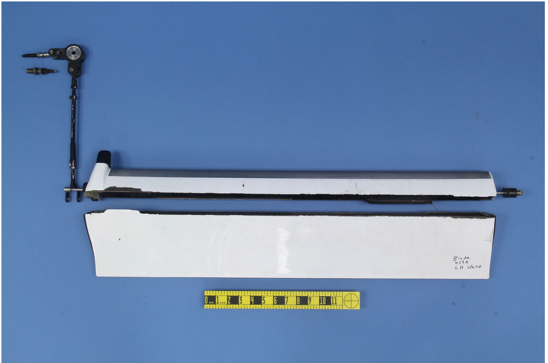
Photo 10 – Left-side, white rotor blade servo flap assembly.
