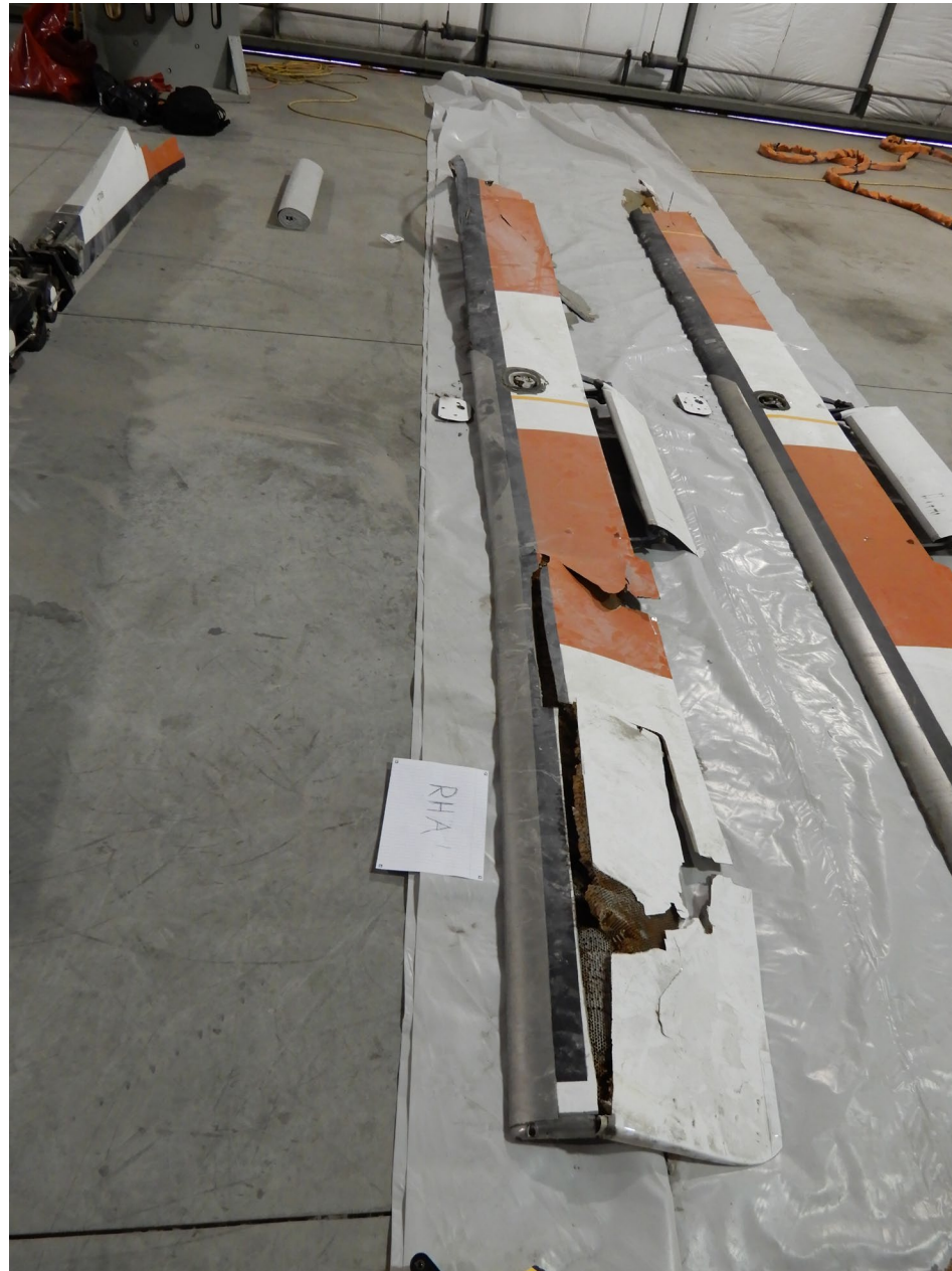
Photo 11 – Right-side white rotor blade as seen from the tip end.
