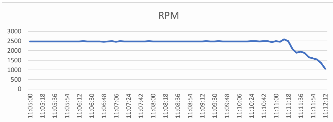
Figure 3-Engine data line chart, last 7 minutes of the flight.
