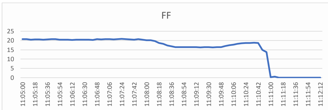
Figure 4-Engine data line chart, last 7 minutes of the flight.
