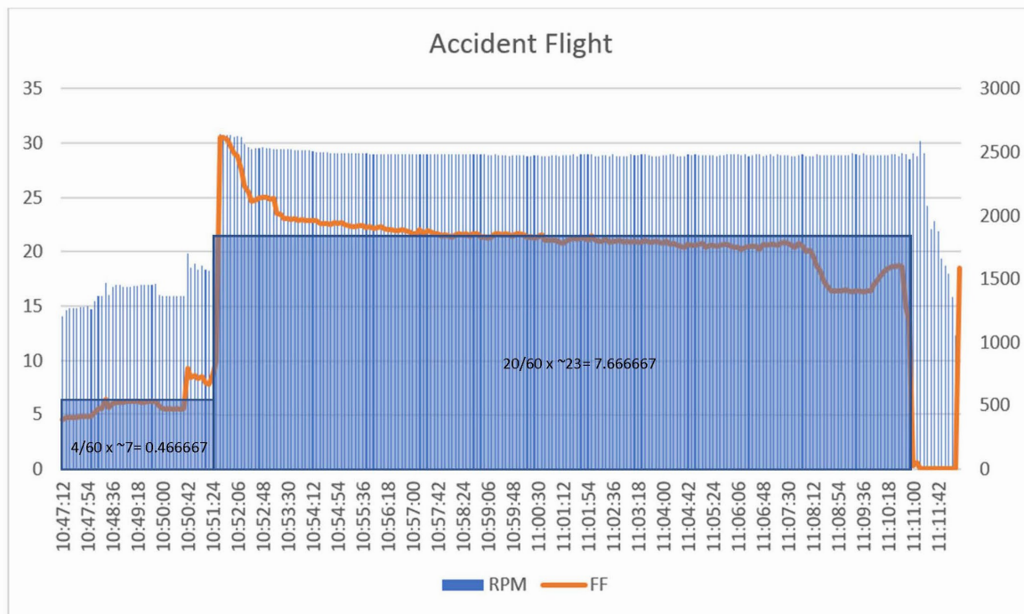
Figure 6-Engine data line chart-fuel consumption rough calculations of complete flight (~8 1/2 gallons).
