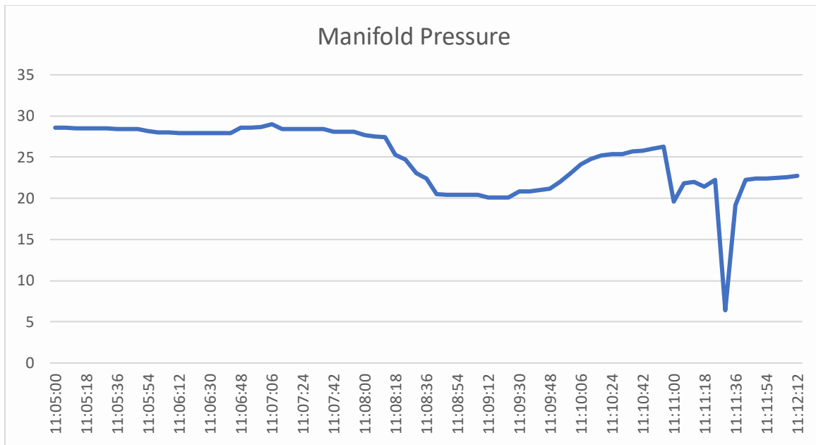
Figure 5-Engine data line chart-last 7 minutes of the flight.
