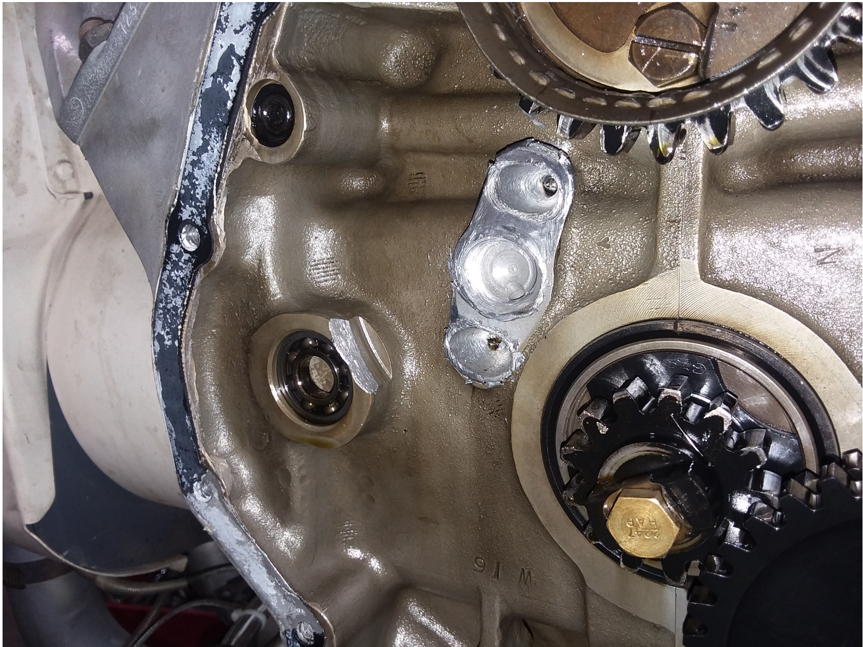
Photo 3 - View of the idler gear and idler gear shaft area and accessory gears. Courtesy of the Federal Aviation Administration.
