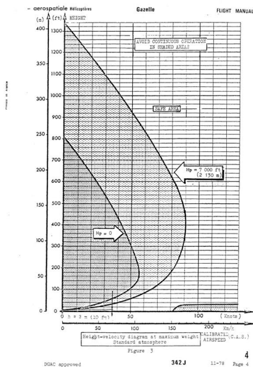
Figure 1. Height/Velocity diagram for the SA-342J helicopter. Image courtesy of Airbus Helicopters.
