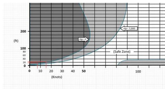
Figure 1. Height/Velocity diagram for the SA-342J helicopter. Image courtesy of Airbus Helicopters.
