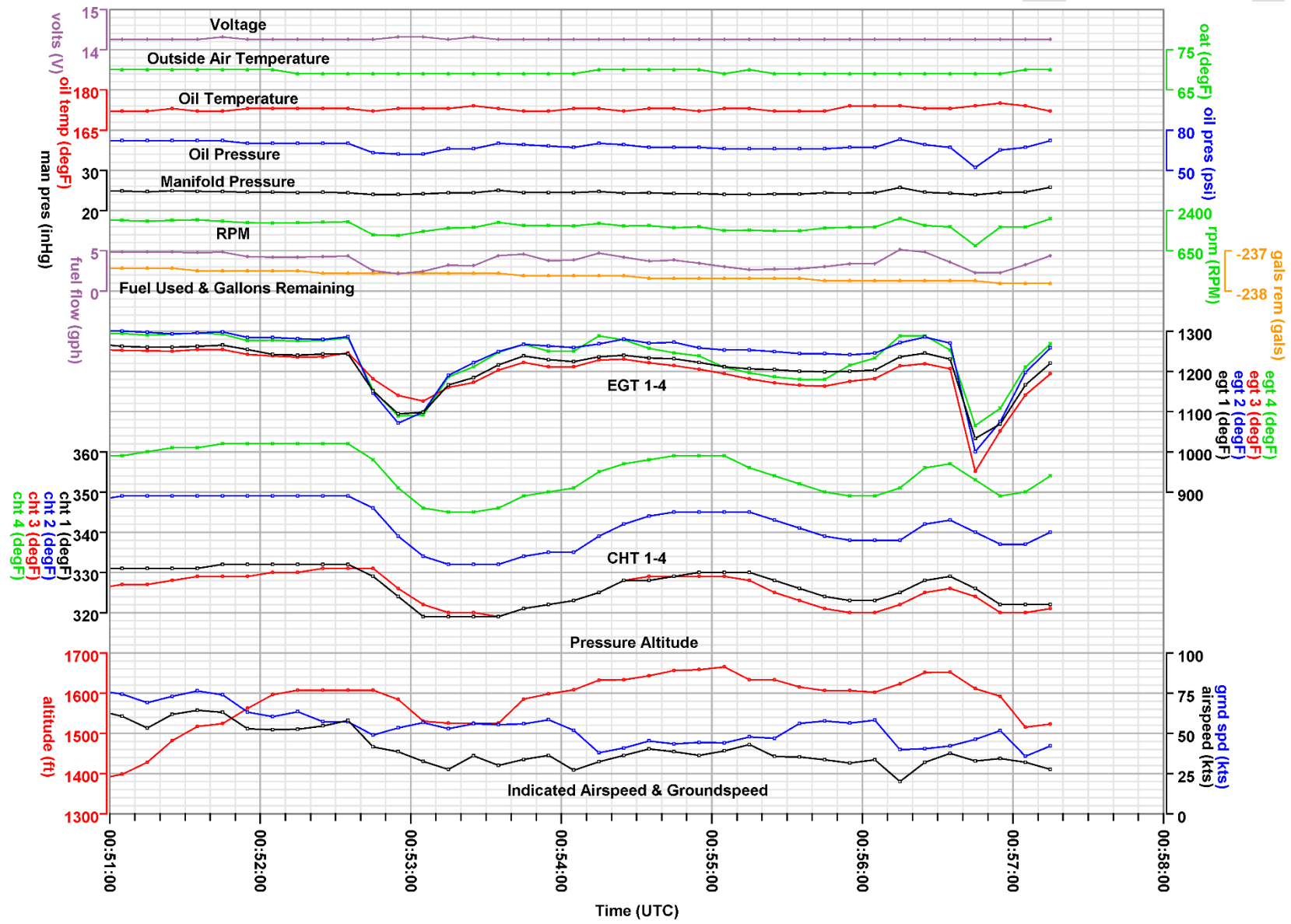
Plot of engine parameters at the end of the accident flight.
