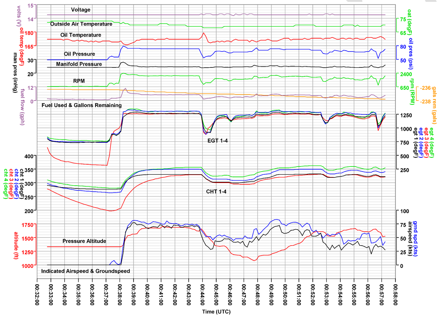
Plot of engine parameters for the accident flight.
