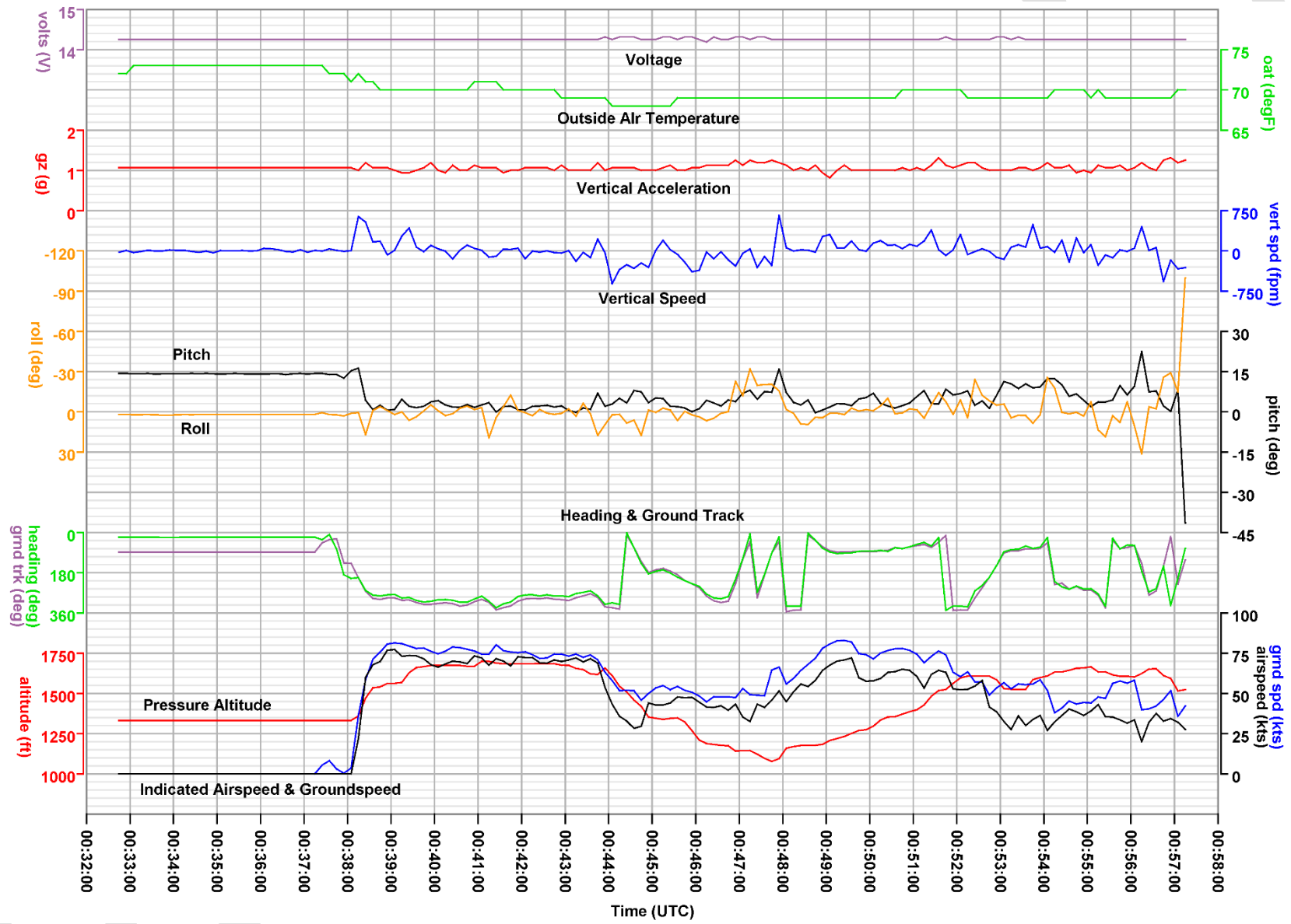
Plot of basic parameters for the accident flight.
