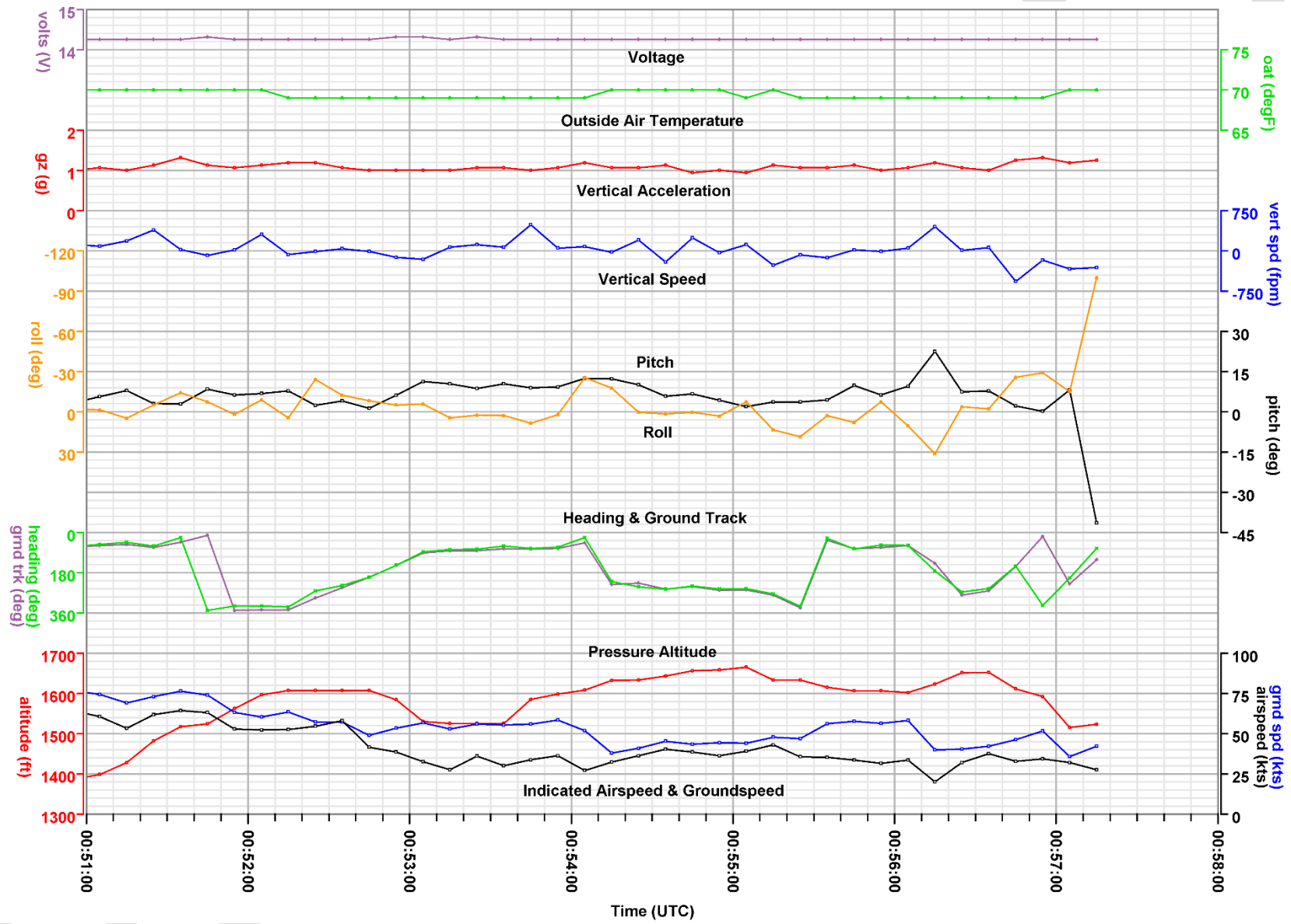
Plot of basic parameters at the end of the accident flight.
