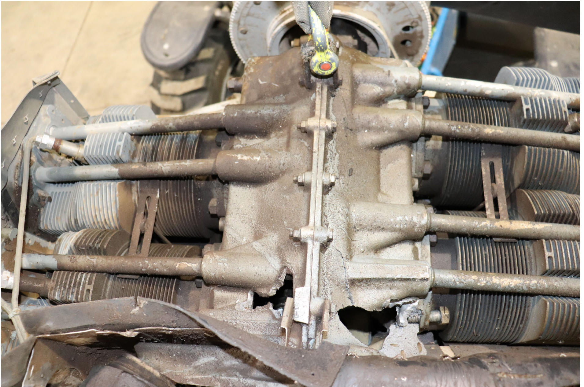
Photo 2 – View of the top side of the engine.
