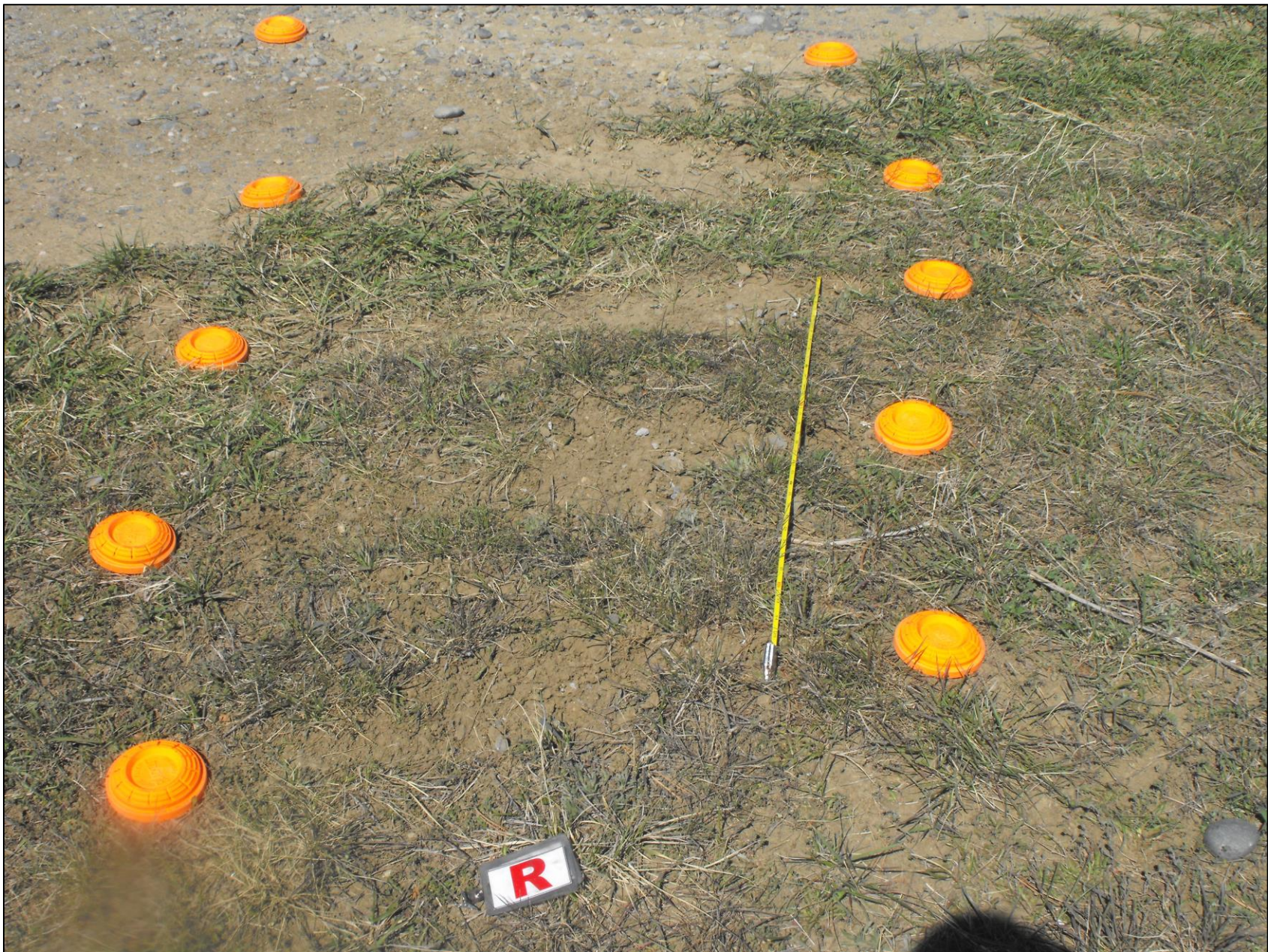
Photo 3 – Accident site, right propeller ground marks. (Courtesy of the FAA)
