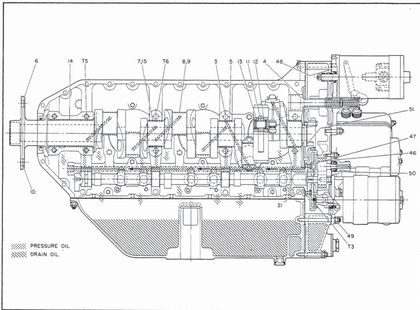
Figure 28. Lubrication Chart, Longitudinal Sectional View (Schematically shown)
