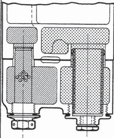
SECTION THROUGH HIGH AND LOW PRESSURE OIL SCREENS
