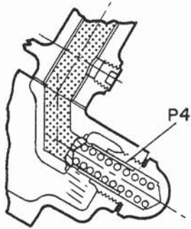
SECTION THROUGH OIL PRESSURE RELIEF VALVE
