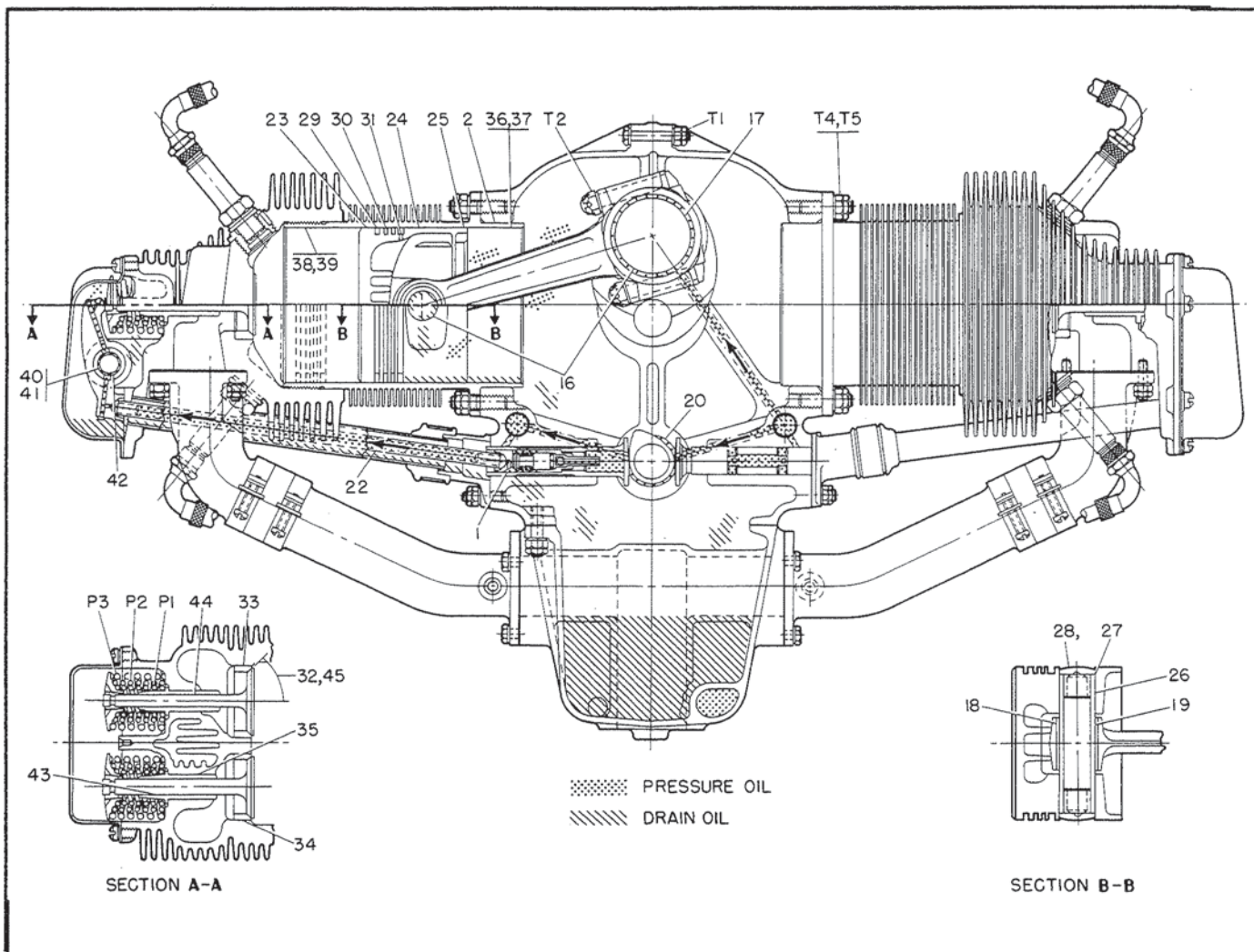
Figure 27. Lubrication Chart, Lateral Section Front View.
