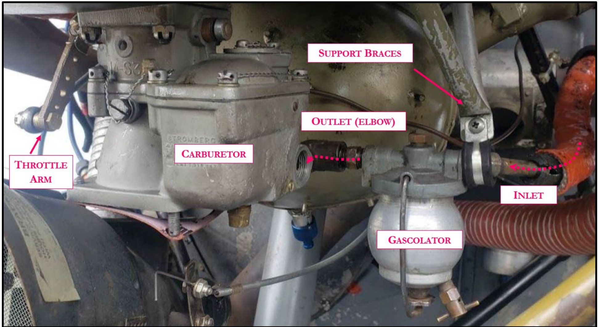
Figure 1: Fuel System
