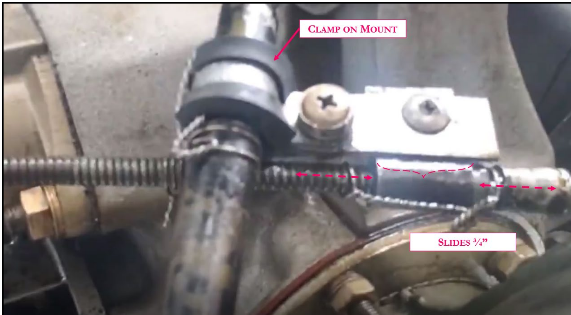
Figure 4: Throttle Cable Clamp
