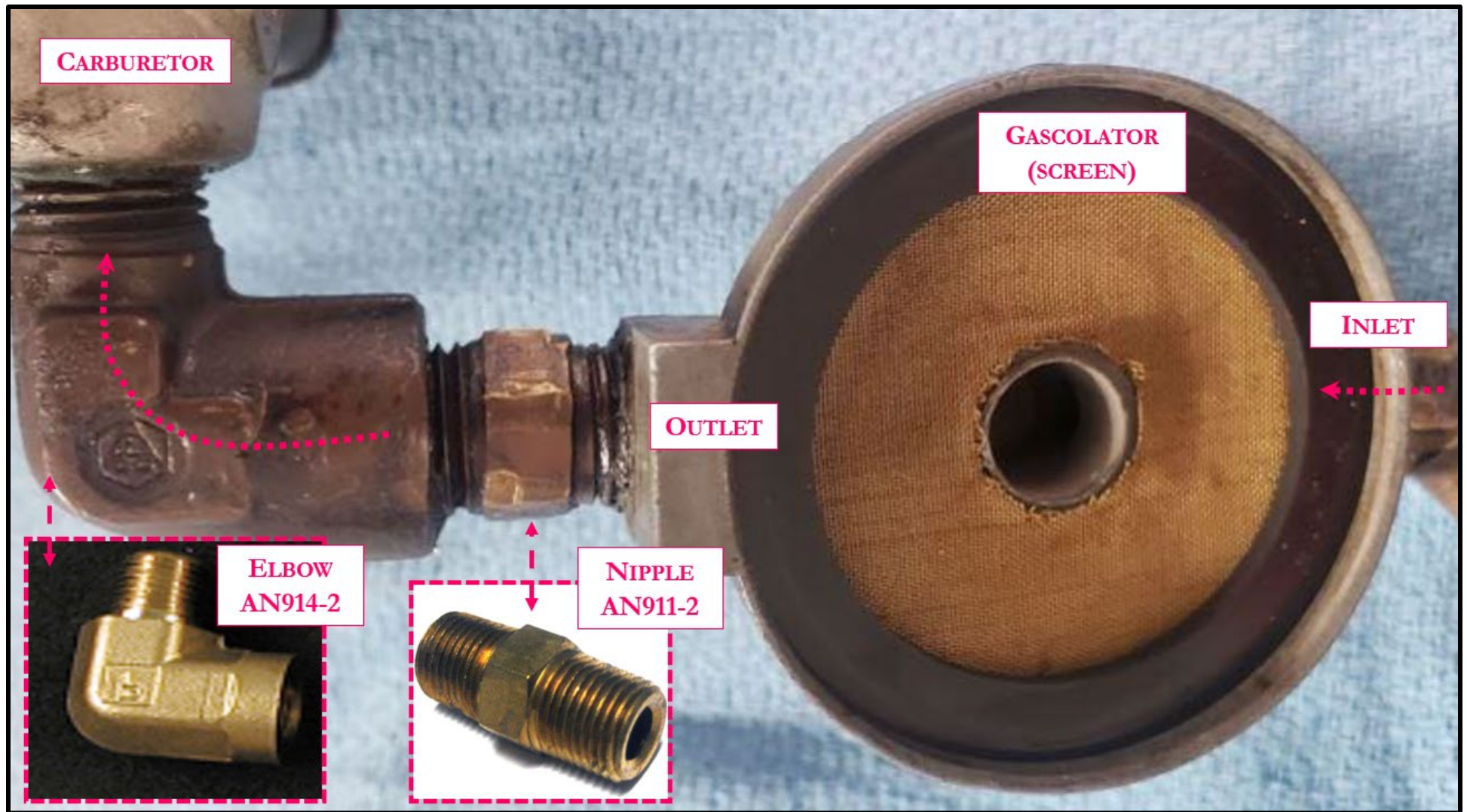
Figure 2: Gascolator
