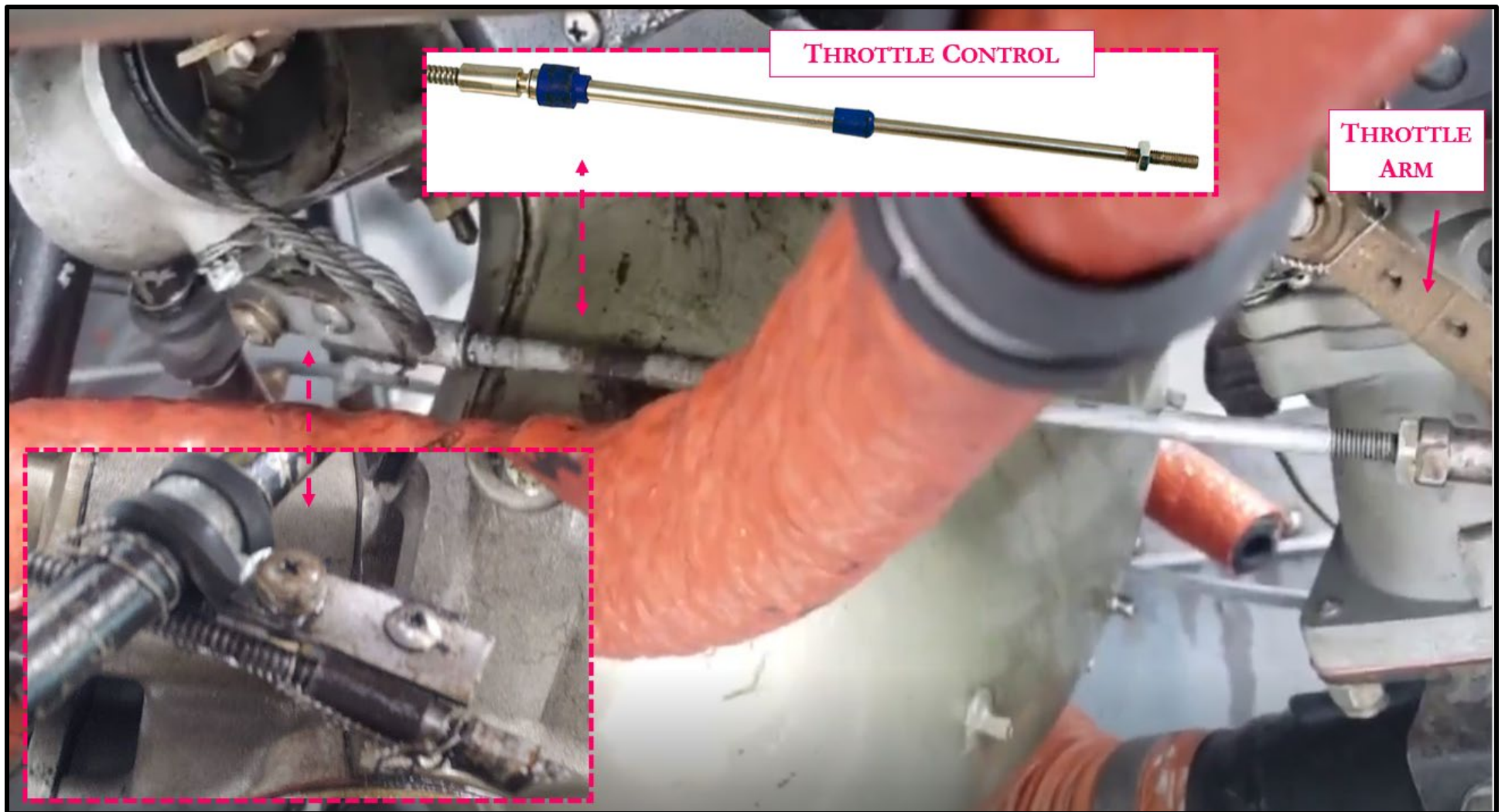
Figure 3: Throttle Cable
