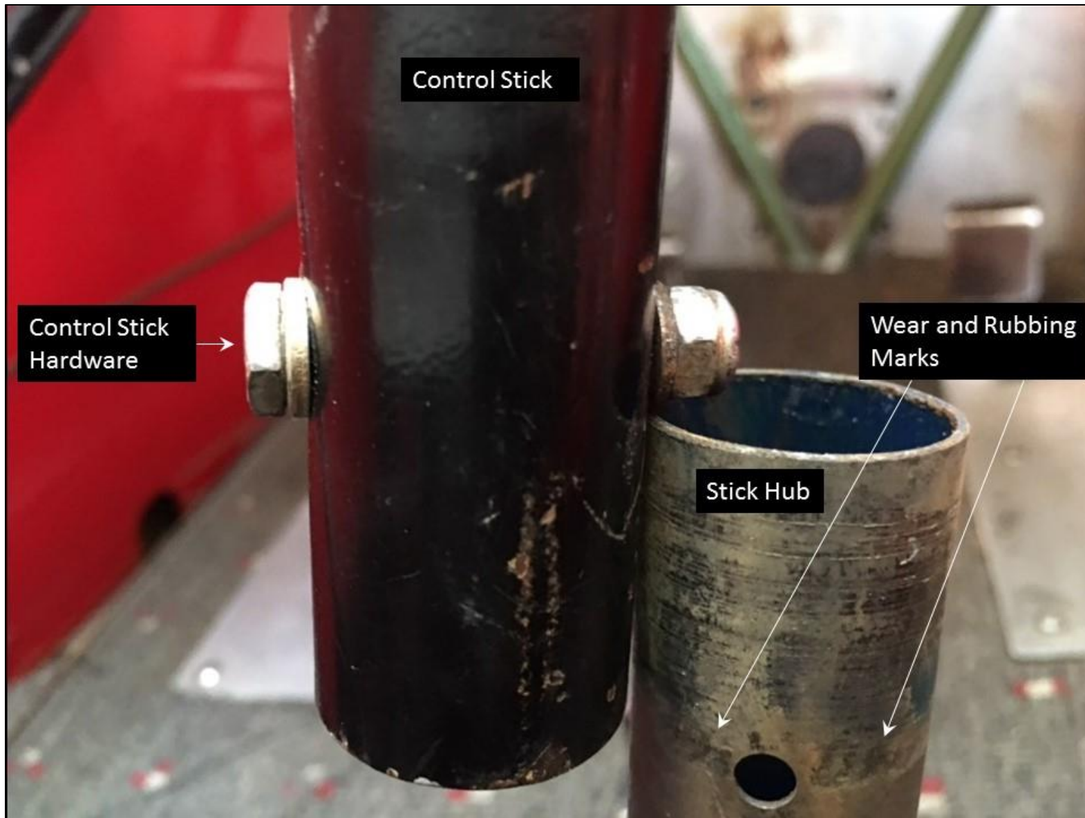
Figure 1-Flight Control Stick and Stick Hub Assembly
