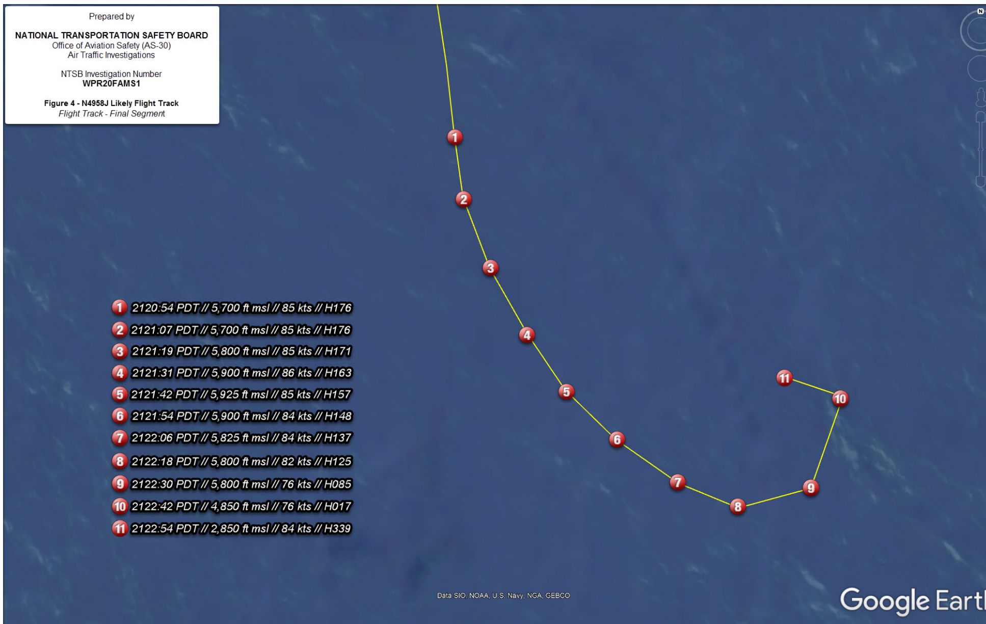
Photo 2 – Flight Track over the Pacific Ocean
