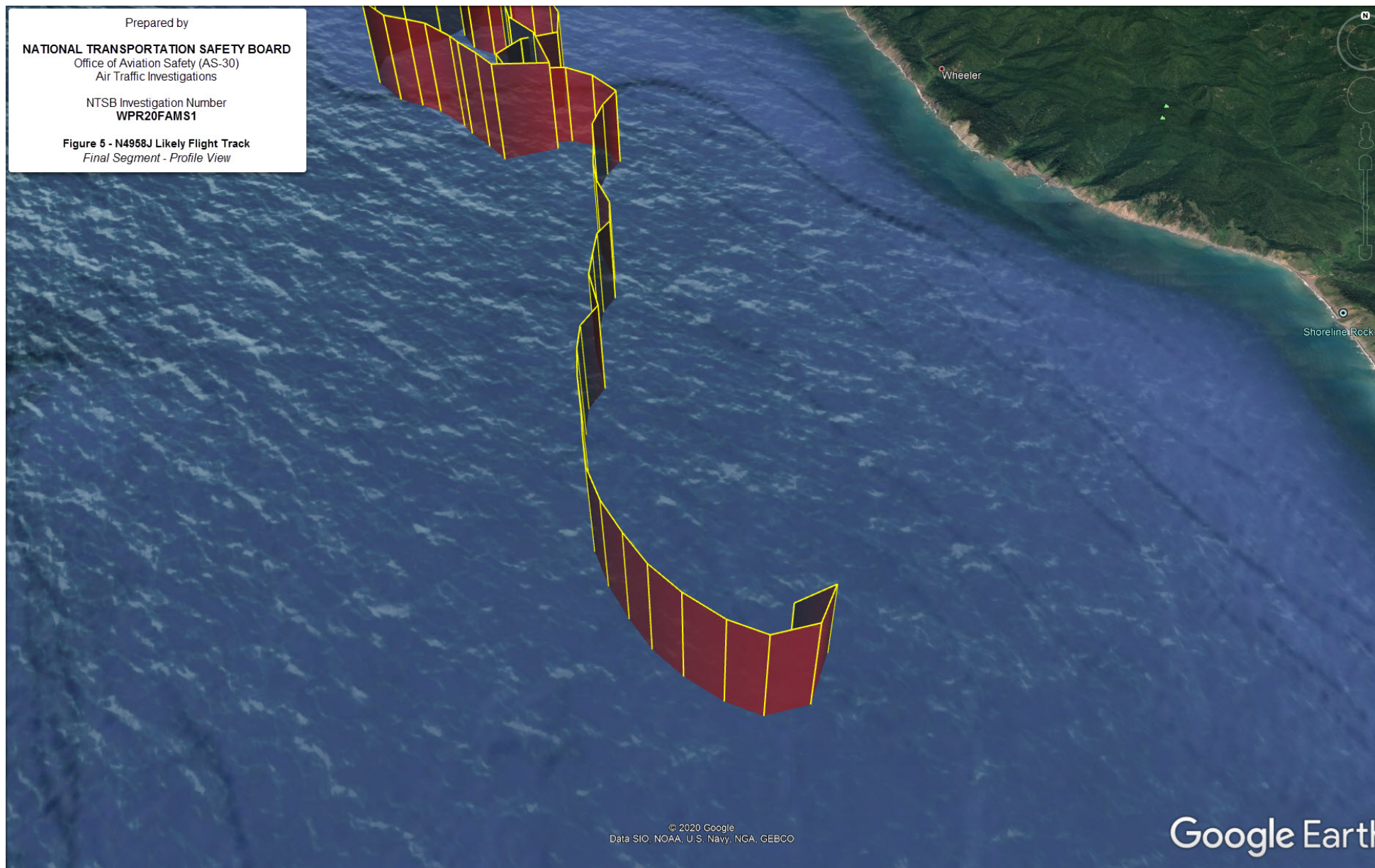
Photo 3 – Flight Track over the Pacific Ocean
