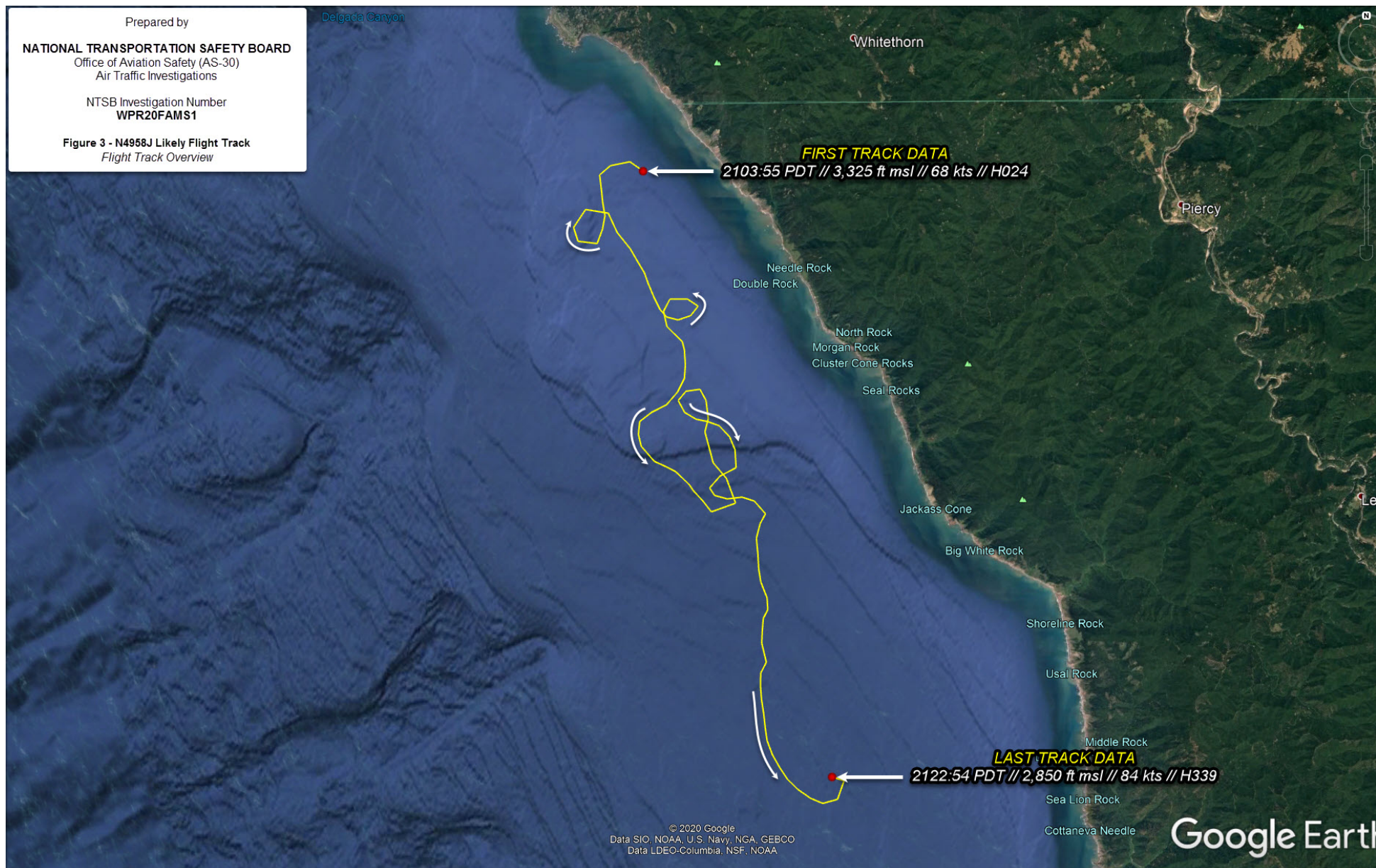
Photo 1 – Entire Flight Path over the Pacific Ocean
