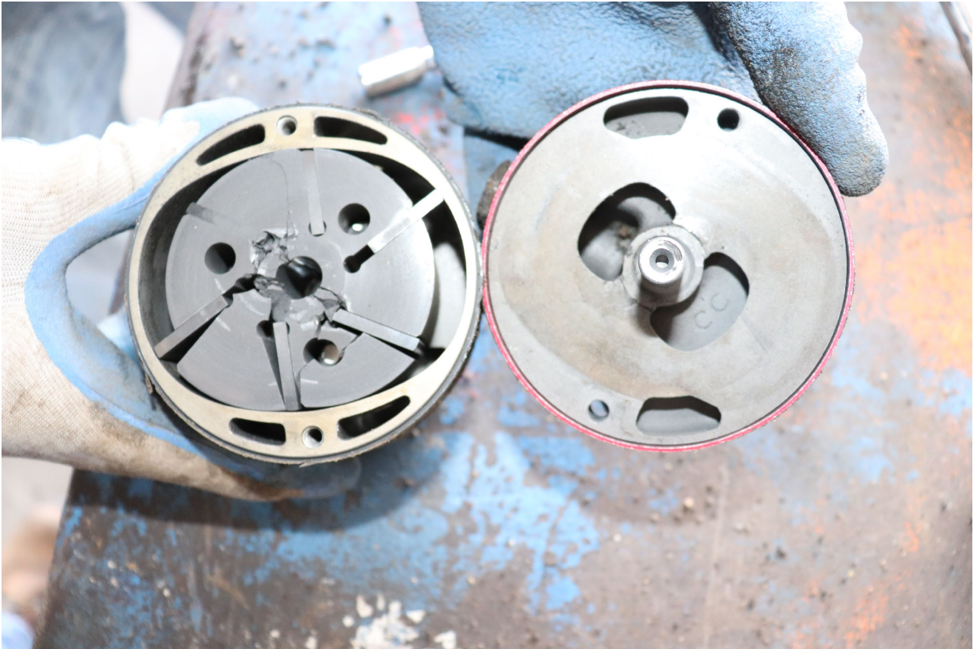
Photo 6 – View of the internal components of the vacuum pump
