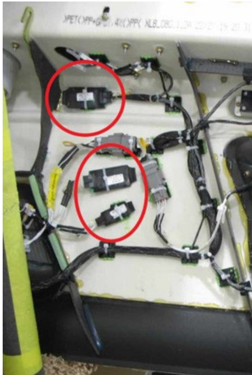
Photo 3 - Audio cards and (smaller) microphone card inside the panel wall (Source: Cirrus).
