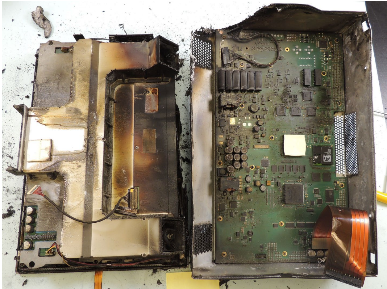
Figure 1 - MFD
