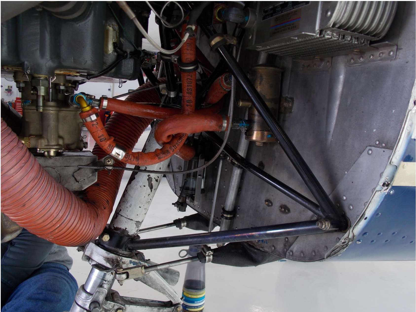
Photo 2 – Engine Mount
