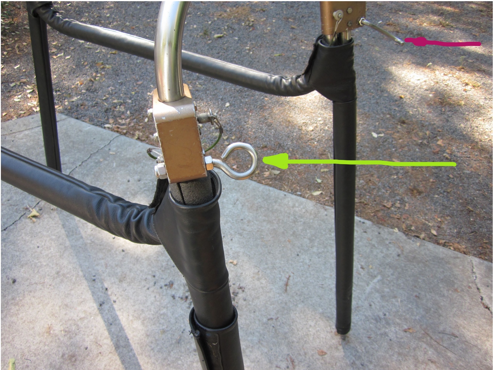
Photo 8 – Close-up View of Eyelet Screws (Photo Courtesy of FAA)
