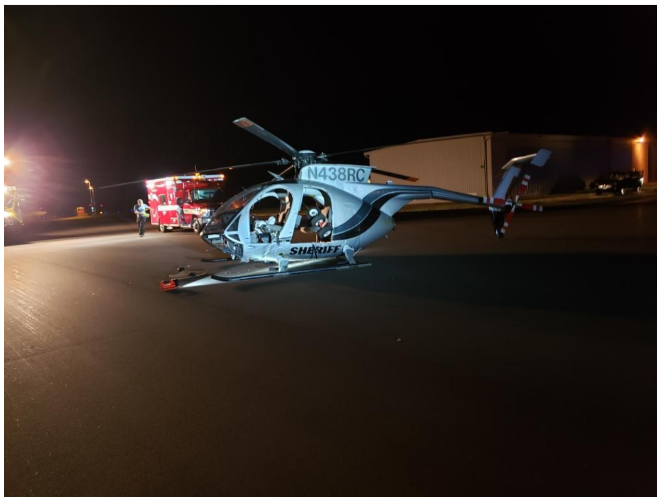
Figure 3: Left Side of Helicopter
