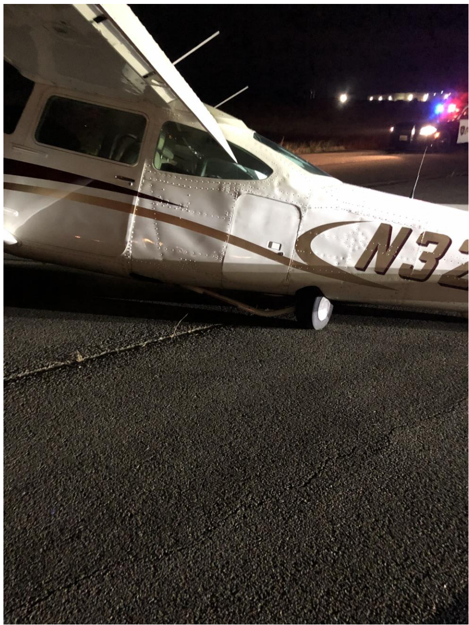
Photo 6 – Accident site, left side view. (Courtesy of the First Responders)
