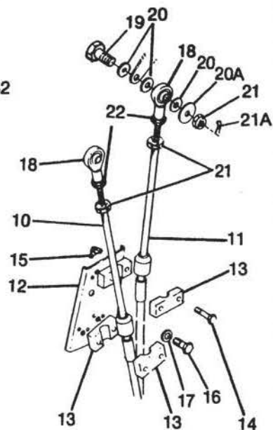
THROTTLE AND MIXTURE CONTROLS
