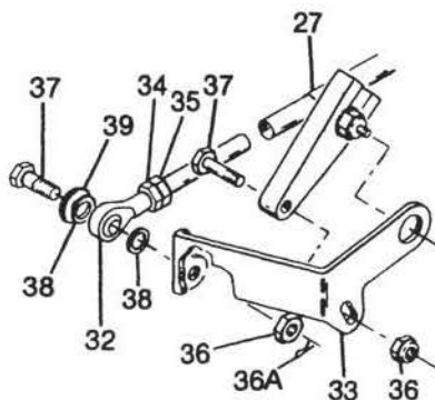
GOVERNOR CONTROL
