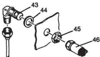
MANIFOLD PRESSURE
