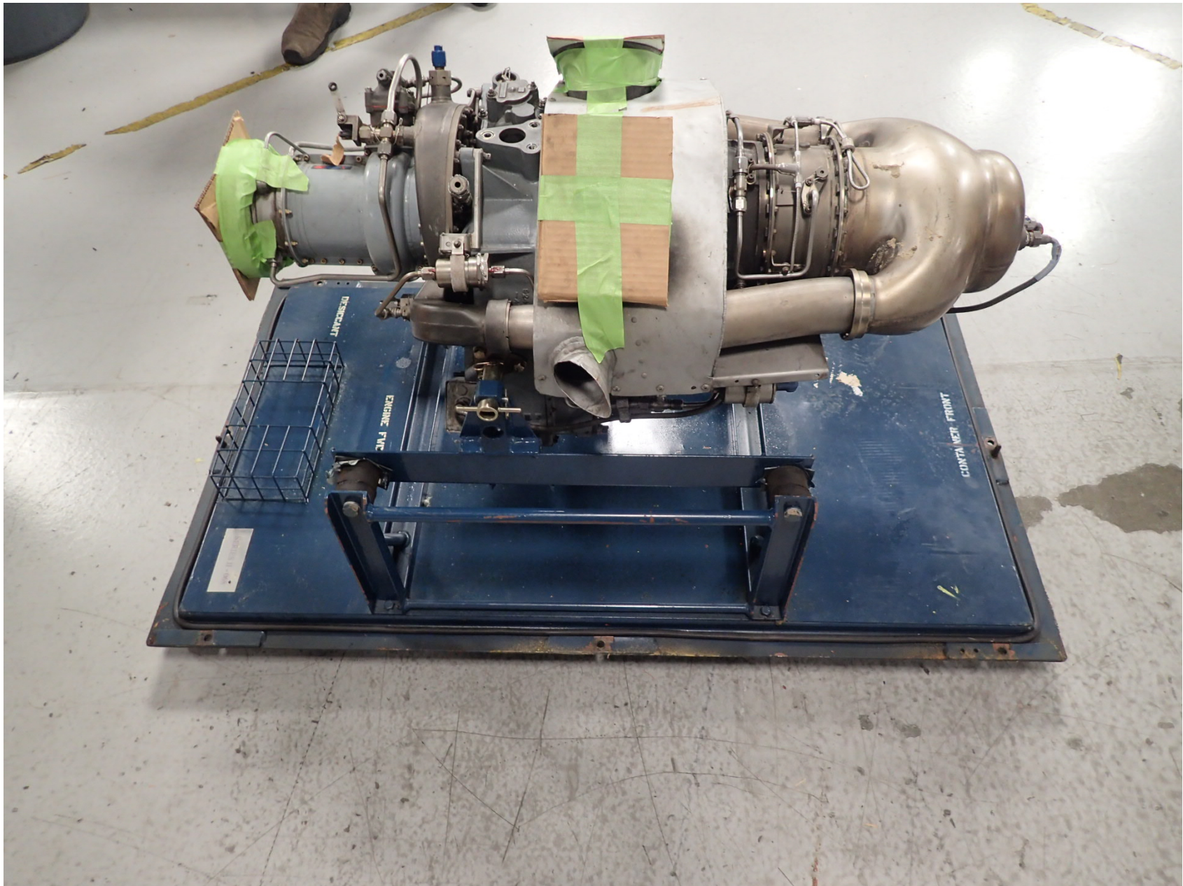
Photo 6 – N3078G Engine Left Side. Photo courtesy of FAA.
