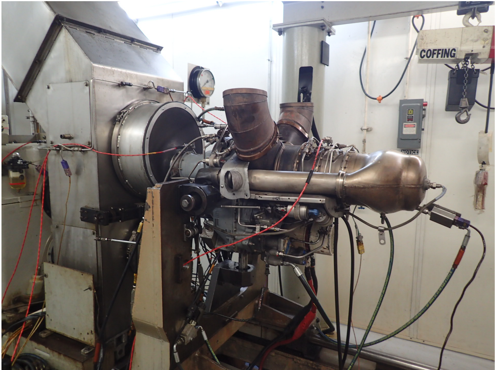
Photo 7 – N3078G Engine Mounted in Test Stand. Photo courtesy of FAA.
