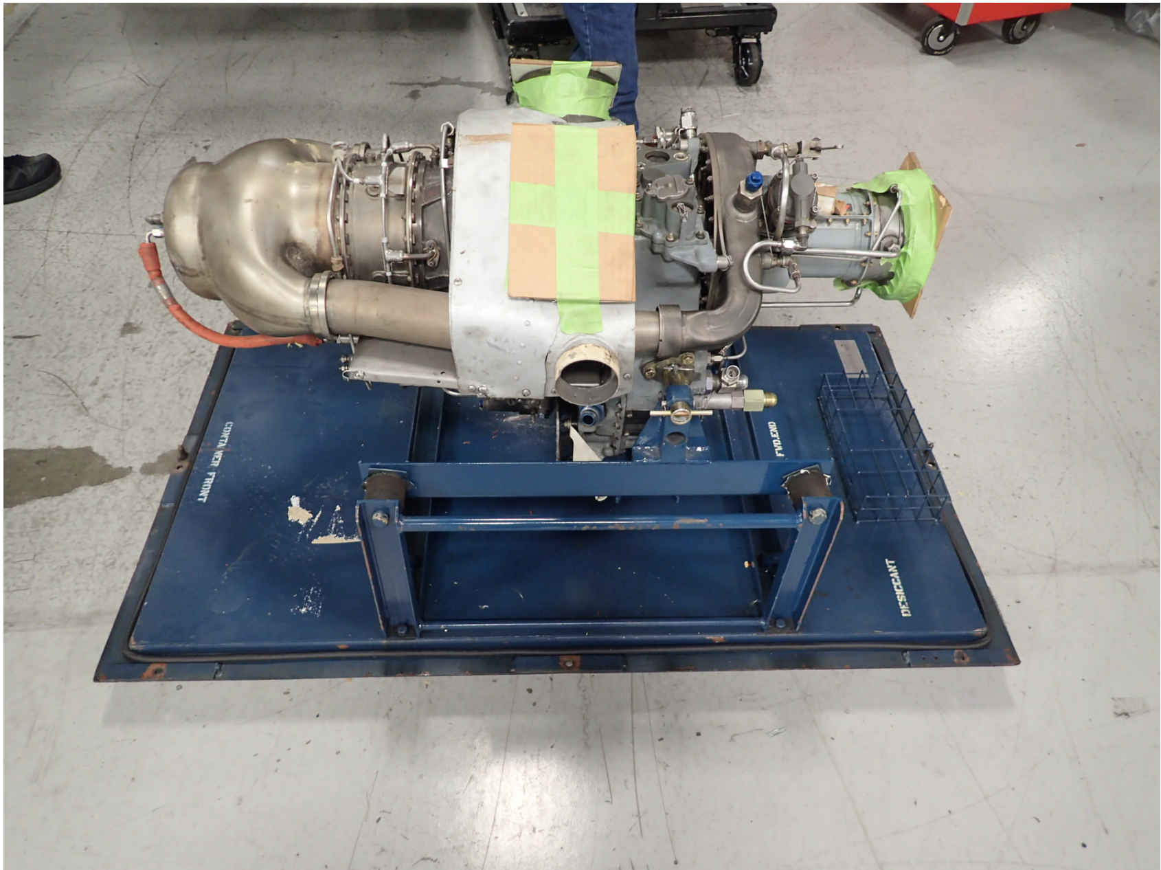
Photo 5 – N3078G Engine Right Side. Photo courtesy of FAA.
