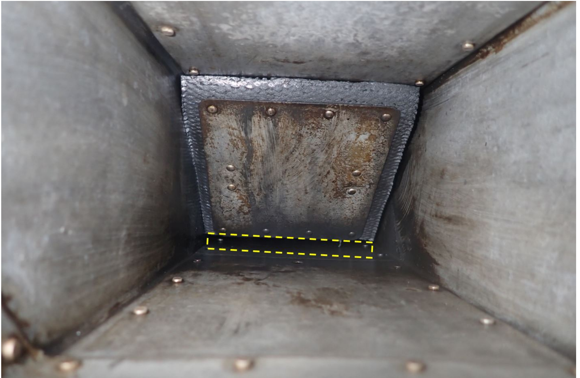
Photo 6 – Carburetor Heat Butterfly Valve with Carb in the Heat ON Position. Viewed from Filtered Air Inlet. Missing Seal Highlighted.
