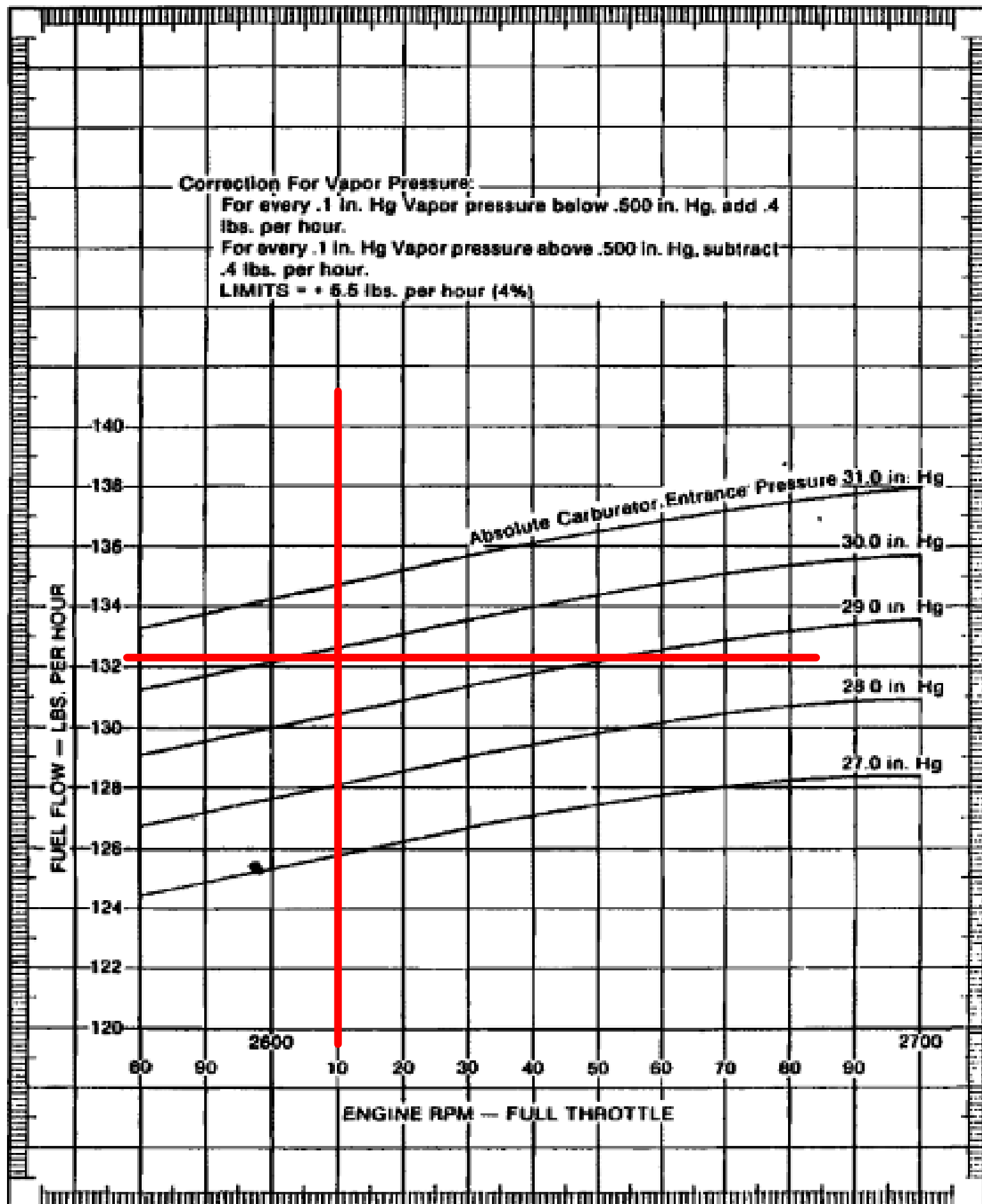
Figure 16. FUEL FLOW LIMITS FOR 0-470-K,L,R&S
